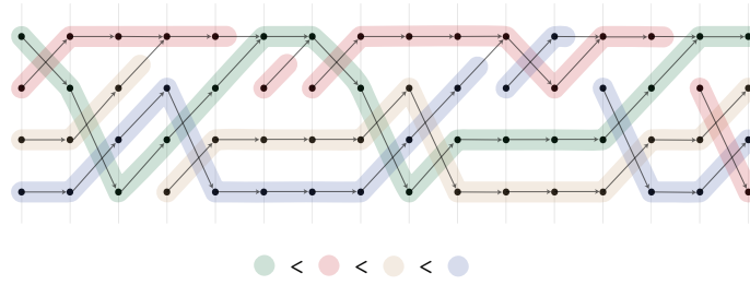
FIGURE 4. Construction of tapes along an input word. The automaton has 4 states and is deterministic. The dots are pairs consisting of a position in the word and a state of the automaton. The arrows denote the transitions of the automaton along the input letters. The colors correspond to the tapes. Every color occurs exactly once at each position, and when following an edge, the color can either remain unchanged or decrease.
