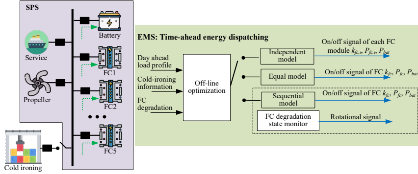
Fig. 4. Overall structure of the proposed EMS
