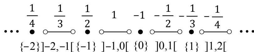
Figure 1. Bijection between G_1 and Z .
