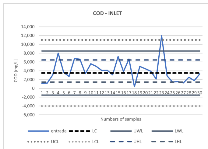
Figure 4. COD inlet.
