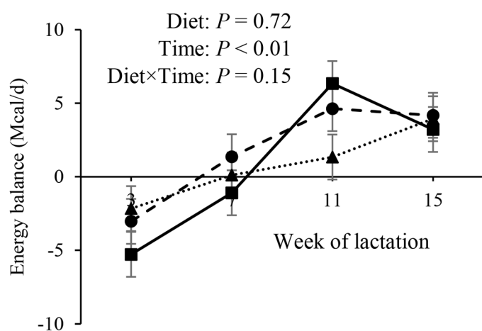
Figure 2. Effect of dietary CLA supplement and higher starch and oil-containing diet (HSO) on energy balance of dairy cows during the first 16 wk of lactation. Control = control diet ( n = 13 , ■ and solid line); CLA = CLA-supplemented diet ( n = 9 , ● and dashed line); HSO = higher starch diet supplemented with sunflower and fish oil (2:1) ( n = 11 , ▲ and dotted line). Error bars represent SEM.
