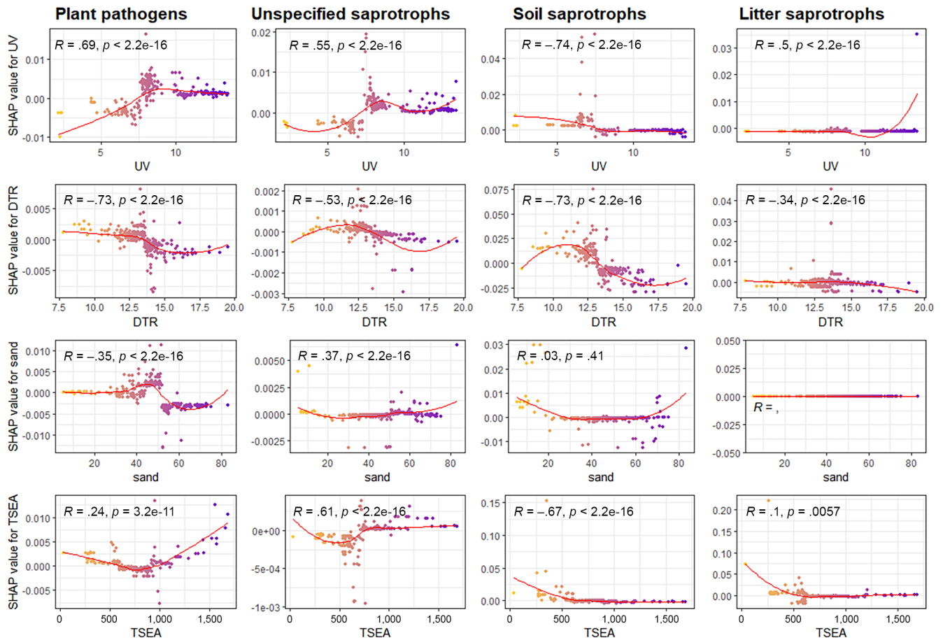
FIGURE 3 Distribution and environmental predictors of the main fungal ecological groups in drylands. Shapley additive explanations (SHAP) dependence plot of selected climatic and edaphic predictors of plant pathogens and saprotrophs richness in drylands. The effects are expressed as SHAP values, which measure the impact of each predictor on the model output (richness of a particular fungal ecological group). SHAP values are derived for a given predictor value in a process analogous to partial dependence plots; thus, each point on the plot corresponds to a prediction in a sample (see Materials and methods). DTR = diurnal temperature range; UV = UV index; TSEA = temperature seasonality; sand = sand content; R = Spearman's rho correlation coefficient; p = p value
