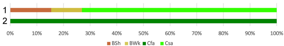
Fig. 4. Köppen-Geiger climate signatures of Parrotia persica and P. subaequalis based on their modern distribution. Climate types according to Kottke et al. (2006), Peel et al. (2007), and Rubel et al. (2017).
