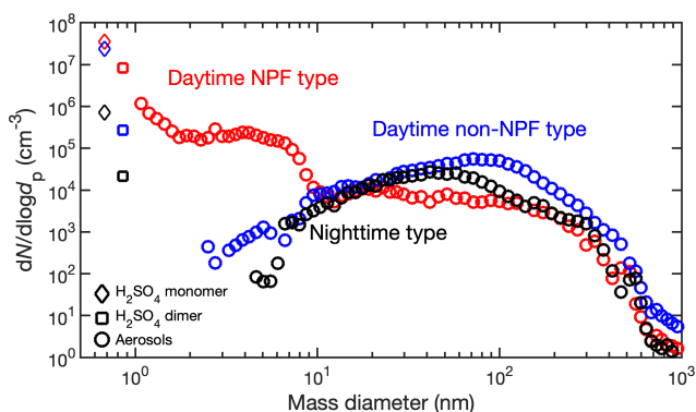
Figure 2. Cases of three typical types of number size distributions from \text{H}_2\text{SO}_4 monomer to dimer and then to larger aerosol size: the daytime NPF type (red), daytime non-NPF type (blue), and nighttime type (black). The daytime NPF, daytime non-NPF, and nighttime particle number size distribution (PNSD) is selected during the NPF period on a NPF day (16 February 2018, 11:10 LT), during the daytime on a non-NPF day (25 February 2018, 12:25) and during the nighttime (4 April 2018, 00:35). The diamonds, squares, and circles represent the distribution function ( dN/d\log d_p ) of \text{H}_2\text{SO}_4 monomers, dimers, and aerosols, respectively.
