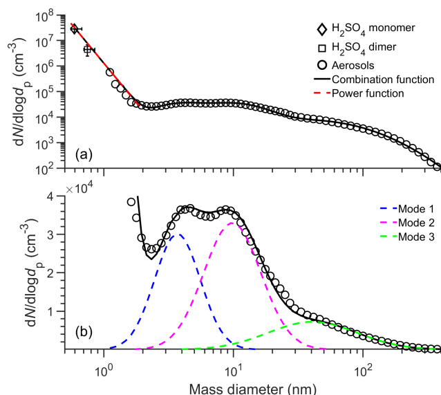
Figure 3. The median daytime NPF type number size distributions from \text{H}_2\text{SO}_4 monomer to larger aerosols and the fitted size distributions shown in (a) logarithmic scale and (b) linear scale of y axis. The x axis error bars of \text{H}_2\text{SO}_4 monomers and dimers indicate the variation range of estimated \text{H}_2\text{SO}_4 monomers and dimers diameters by assuming the bulk density to be 1000–1800 \text{kg m}^{-3} . The y axis error bars of \text{H}_2\text{SO}_4 monomers and dimers indicate the 25th–75th range of concentrations. The black and red lines indicate the fitted size distribution in the whole size range and in sub-3 nm size range, respectively. The blue, magenta, and green lines present the fitted mode 1, mode 2, and mode 3, respectively. The diamonds, squares, and circles represent the distribution function ( dN/d\log d_p ) of \text{H}_2\text{SO}_4 monomers, dimers, and aerosols, respectively.
