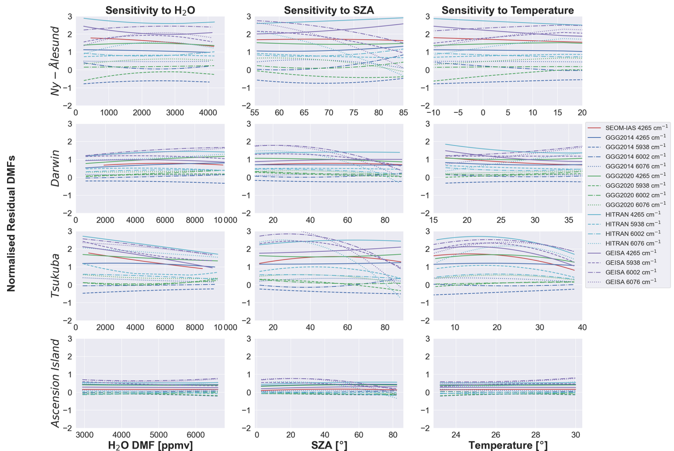
Figure 9. The sensitivity of water vapour, SZAs and temperature variations in retrieved ^{12}\text{CH}_4 DMFs from each TCCON site, spectroscopic database and window. Each subplot shows the second-order regression fit of the normalised residual between the retrieved window and spectroscopic database DMFs and the TCCON reference DMFs, with the fit window and spectroscopic database indicated by the legend. Each row of the figure shows data from each TCCON site as indicated in the y axis, and each column shows the sensitivity to a specific condition as shown in the title.
