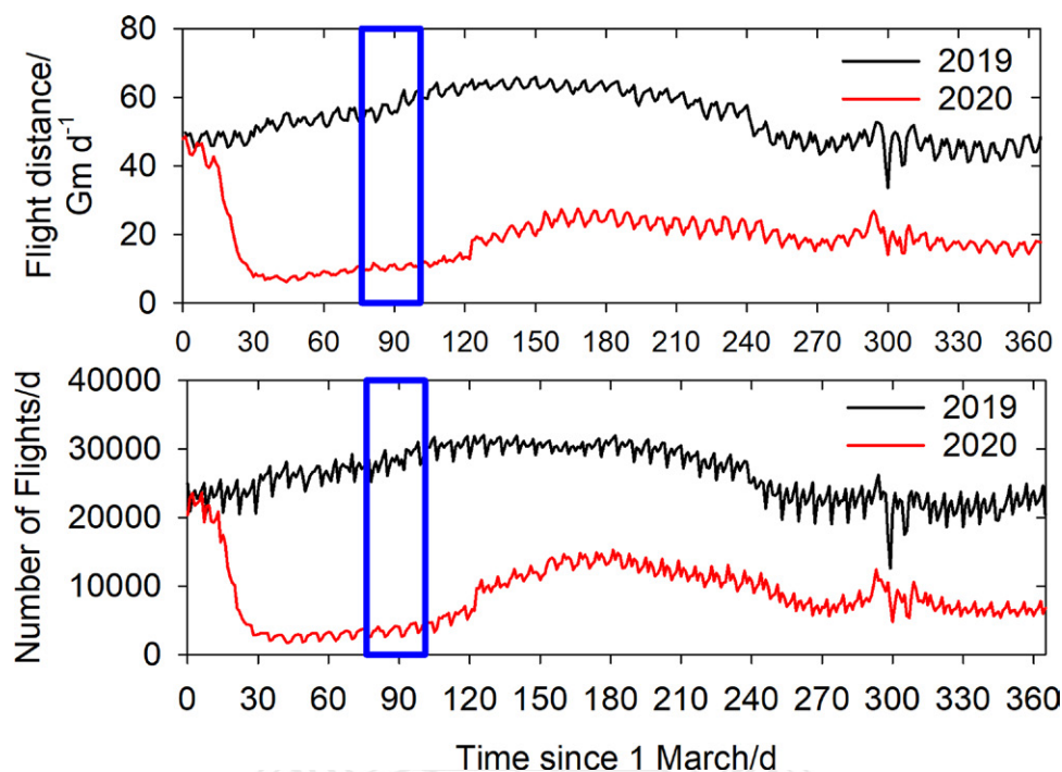
Fig. 2. Flight distance and number of flights over in Europe since 1 Mar 2020 (red) and 1 Mar 2019 (black) from EUROCONTROL and NATS. The BLUESKY period was from 16 May to 9 Jun 2020 indicated by the blue box.
