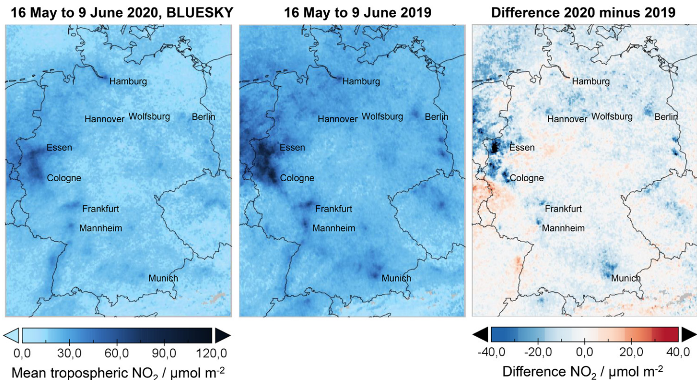
Fig. 8. Mean tropospheric \text{NO}_2 vertical column densities over Germany for (left) 2020 and (middle) 2019 averaged over the BLUESKY period from 16 May to 9 Jun. The means were derived from Sentinel-5P/TROPOMI level 2 data. (right) The difference of 2020 minus 2019.
