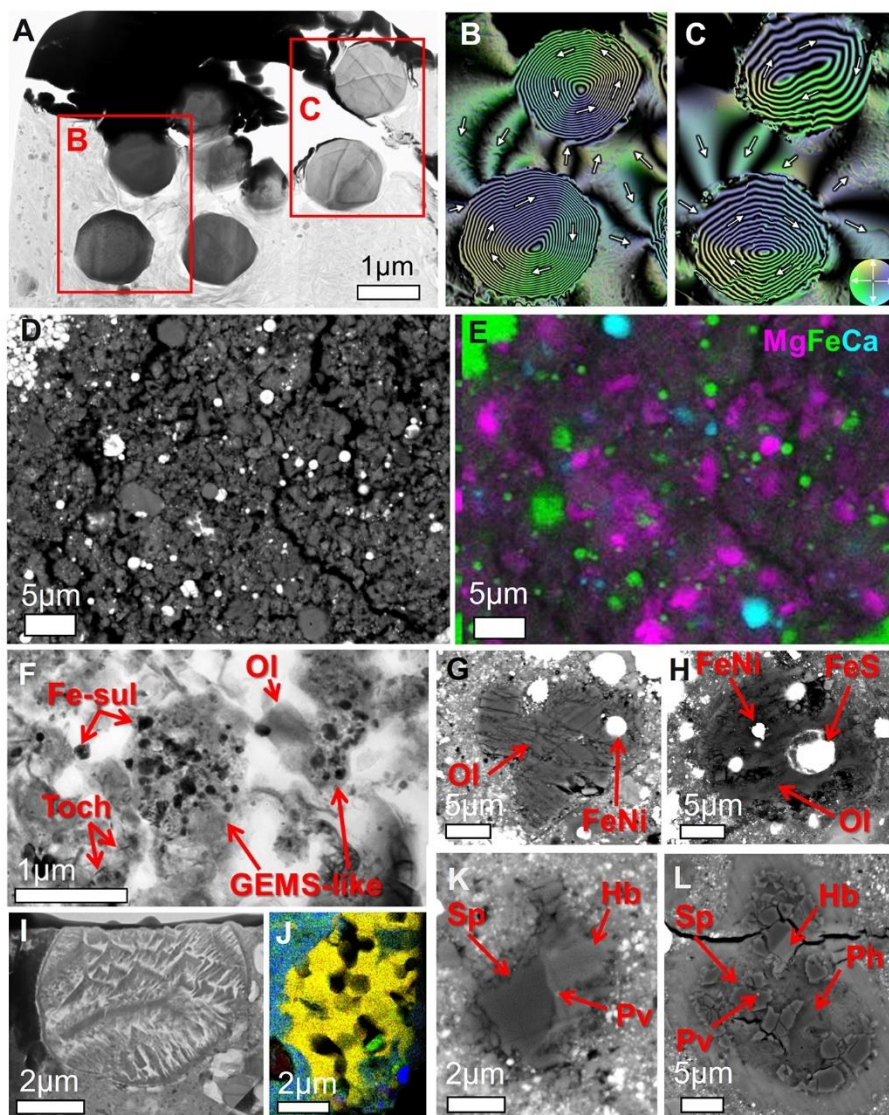
Fig. 3. Characteristic textures, magnetic structures, and embedded objects in the Ryugu samples. (A) TEM image of typical magnetite framboids (dark-grey rounded objects) from A0064. The light-grey area is phyllosilicate from the major lithology, and the upper black area is tungsten contamination. (B and C) Color maps of the magnetic flux direction obtained from the reconstruction of remanent magnetism, for the magnetite framboids in red boxes in panel A observed using electron holography (7). Each particle has a concentric circular magnetic field (vortex structure) indicated by white arrows, which show the direction of the magnetic flux as shown in the color-wheel in panel C. Figure S5 shows the composition and electron diffraction data for this region. (D) Enlarged view of the least-altered fragment 4 in sample C0002, showing high porosity. (E) Compositional map of panel D, showing high abundances of Mg-rich olivine and Mg-rich low-Ca pyroxene (magenta), magnetite and pyrrhotite (green), and minor Ca carbonate (light blue). (F) TEM image of a part of the least-altered fragment 5 in C0002, showing a very porous aggregate with labeled GEMS-like objects, Fe sulfide (Fe-sul), Mg-rich olivine (OI), and tochilinite (Toch). (G to I) Chondrule-like objects. Objects in panels G and H, both from C0002, show textures similar to type-I chondrules, consisting of Mg-rich olivine (OI) and an FeNi metal inclusion. An FeS inclusion occurs only in panel H. The object in panel I, from C0076, shows a barred-olivine texture, consisting of several sets of parallel olivine bars and an olivine rim. (J) TEM/energy-dispersive spectrometer (EDS) color map of a porous olivine (yellow) from C0076, including a small Al, Ti-rich diopside crystal (green). RGB colors indicate the concentration of Mg, Si, and Fe, respectively. (K and L) Small CAIs-like objects. The object in panel K, from C0040, consists of Al spinel (Sp), hibonite (Hb), and a small inclusion of perovskite (Pv). The object in panel L, from C0002, consists of Al spinel (Sp), hibonite (Hb), a small inclusion of perovskite (Pv) and phyllosilicate (Ph). Panels A, F, I are bright-field TEM images and panels D, G, H, K, L are BSE images.
