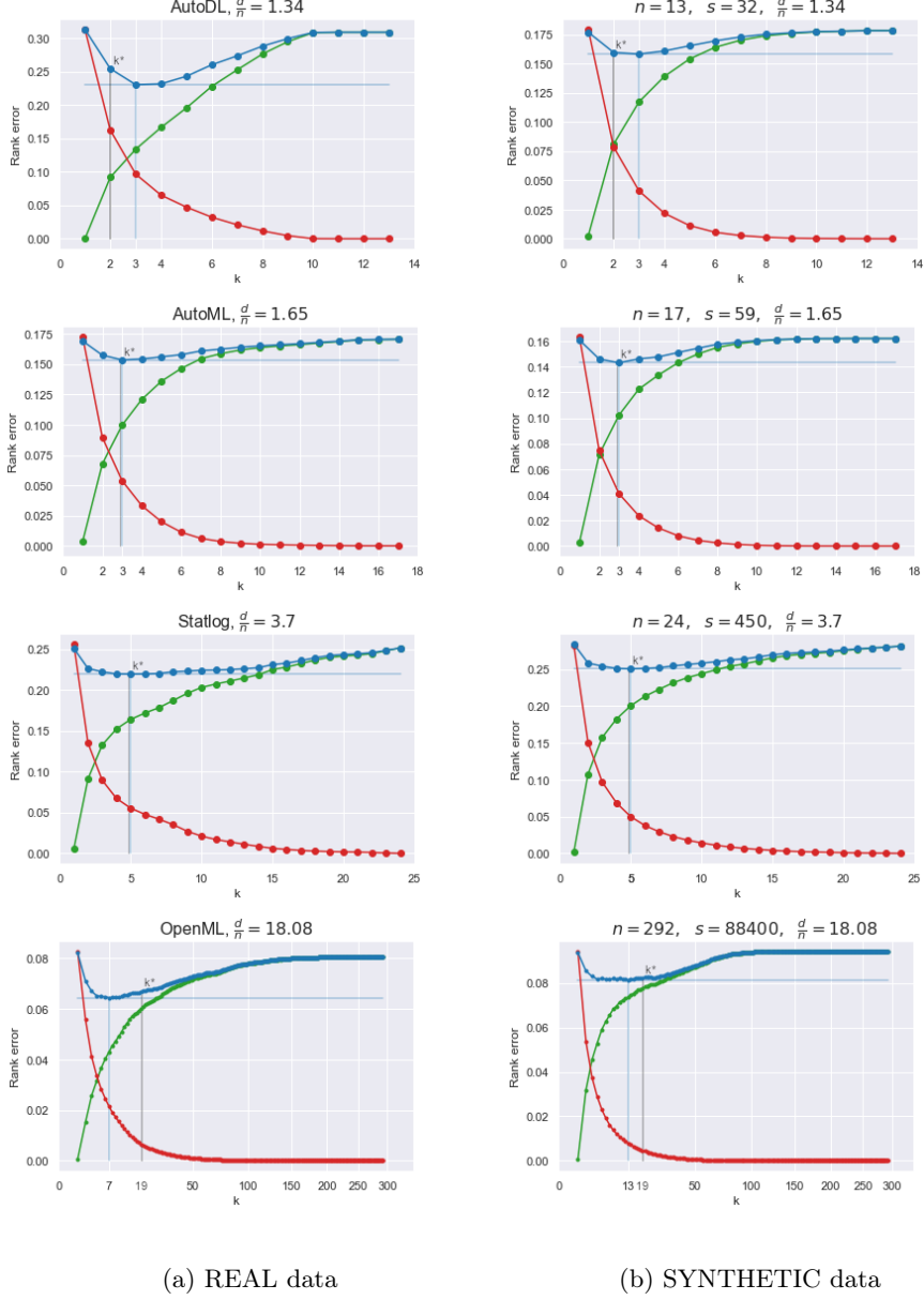
Fig. 1: Learning curves with top-k method (averaged over 10000 trials): Meta-training error , Meta-test error , Generalization gap . Rank error is the rank r of the selected winner in \mathbf{F} and \mathbf{P} , normalized by (r - 1)/(n - 1) . The blue vertical bar marks the optimum, s is the number of random swaps, d is the average Kendall \tau distance [6] between phase rankings, and the grey vertical bar marks k^* \simeq 1 + \frac{d}{n} , an estimation of the optimal value of k .
