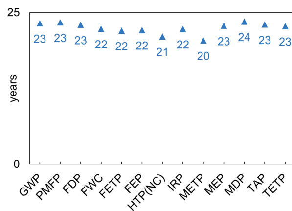
Fig. 12 Operating time of a PST module at which its environmental impact per kW h is equal to that of an SHJ module that has been operated for 25 years.
