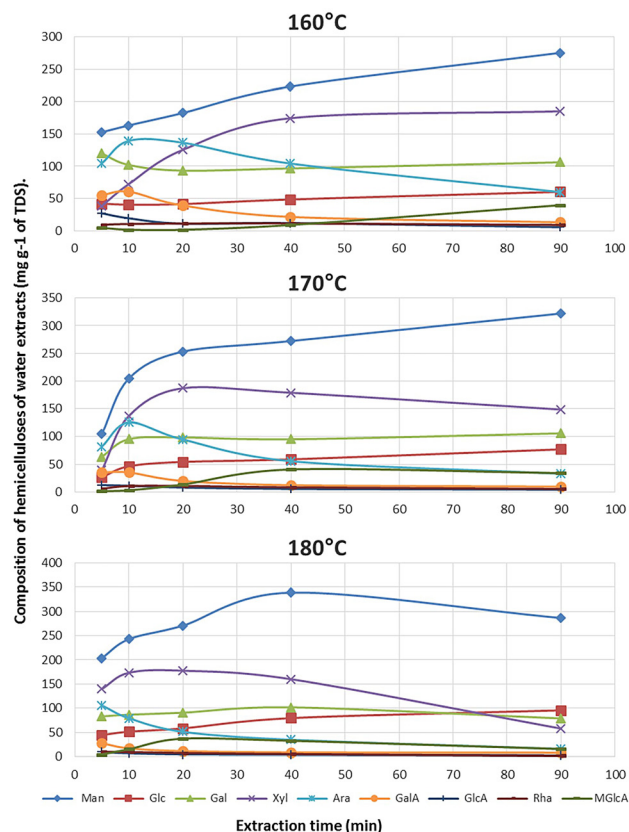
Figure 4: Amounts and composition of hemicelluloses of water extracts obtained at different temperatures ( \text{mg g}^{-1} of TDS).
