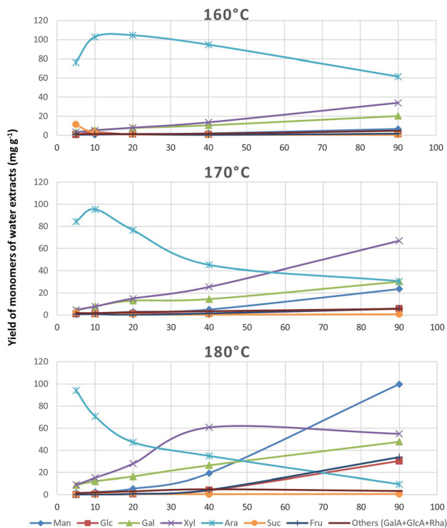
Figure 5: Amounts of monomers of water extracts obtained at different temperatures ( \text{mg g}^{-1} of TDS).
