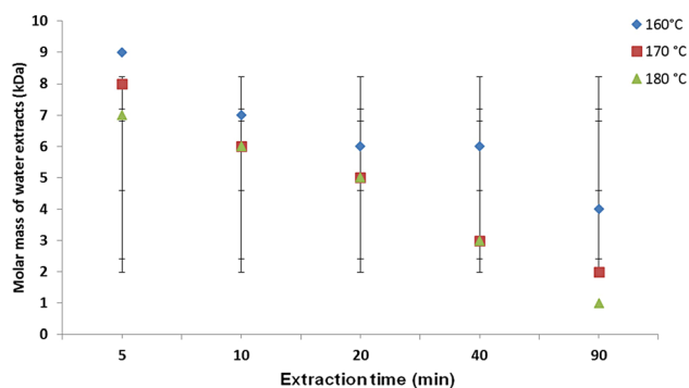
Figure 3: Molar mass of water extracts obtained at different temperatures (kDa).
