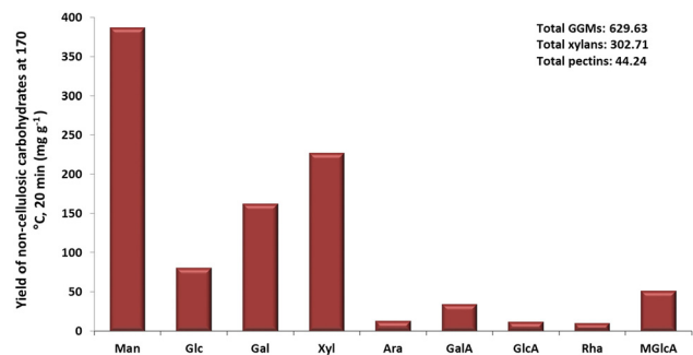
Figure 15: Non-cellulosic carbohydrates obtained at 170 °C, 20 min (mg g -1 of ethanol precipitates).
