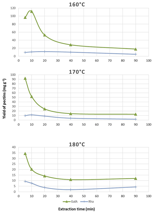
Figure 13: Carbohydrate composition of pectins obtained at different temperatures (mg g -1 of ethanol precipitates).
