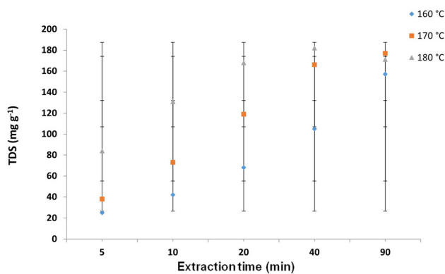
Figure 1: Total dissolved solids (TDS) of water extracts obtained at different temperatures ( \text{mg g}^{-1} of wood).
