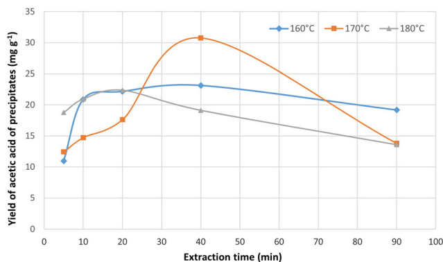
Figure 14: Acetic acid from alkaline hydrolysis of precipitates obtained from water extracts at different temperatures (mg g -1 of ethanol precipitates).
