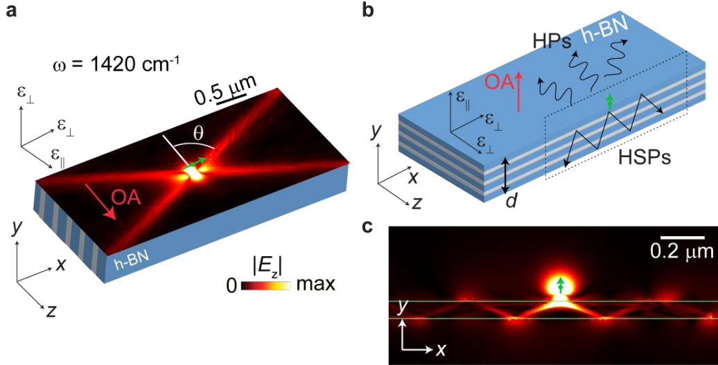
Figure 2.7: Launching of HSPs at the interface between h-BN and air (a) Electric dipole source (green dot and arrow) launching hyperbolic surface polaritons at the interface between h-BN and air, at a frequency \omega = 1420 \text{ cm}^{-1} . The OA is oriented parallel to the surface (red arrow). Color plot indicates |E_z| . (b) Schematics showing the launching of HSPs and HVPs by an electric dipole located near the edge of the thin film with a thickness d = 100 \text{ nm} . The OA is oriented in the y -direction. The dotted rectangle indicates the plane near the edge of the flake where the fields in (c) were calculated. (c) Zig-zag pattern created due to the launching of HSPs by a dipole source at the edges of the h-BN flake. Color plot represents |E_z| . The green dot and arrow represents the dipole source. The layered atomic structure of h-BN is indicated in (a) and (b) by the alternating blue and white colors.
