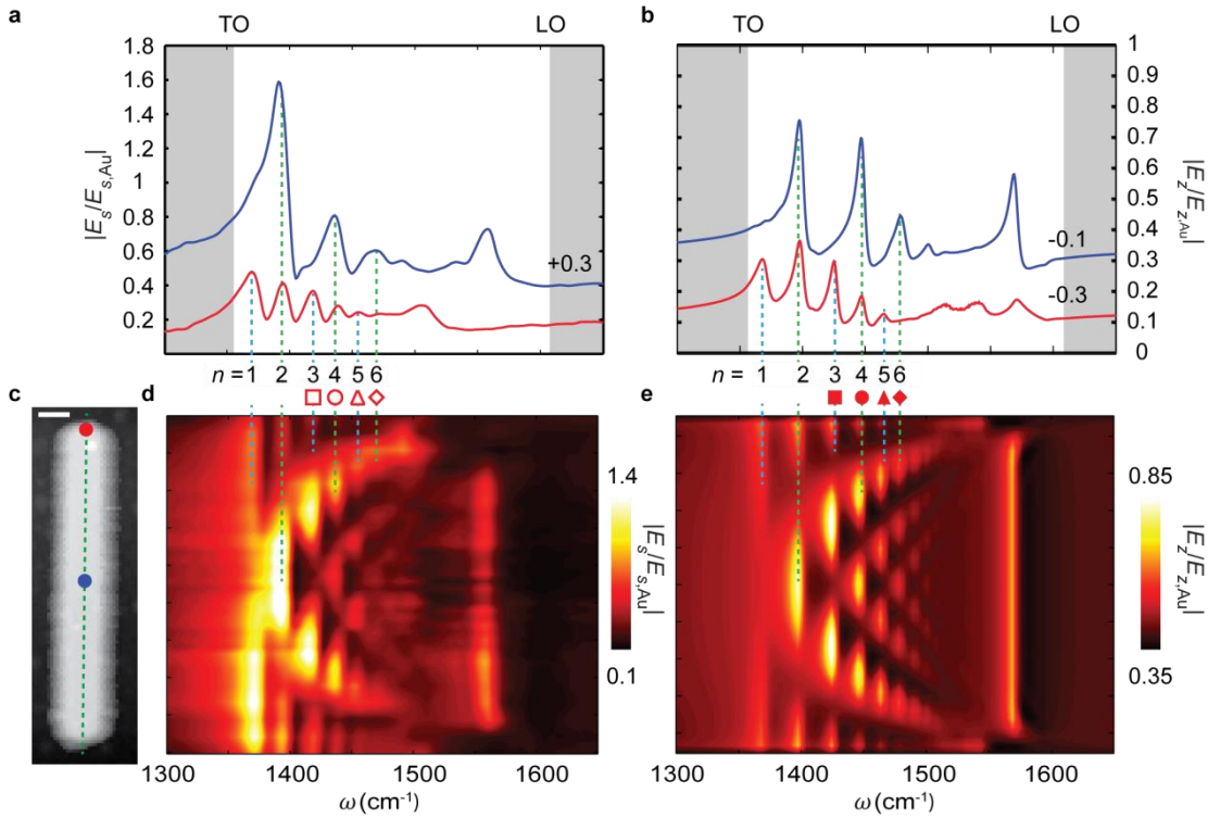
Figure 3.5: Nano-FTIR study of a 1.723 nm long h-BN antenna on SiO 2 . (a) Experimental and (b) simulated nano-FTIR amplitude spectra. They were obtained at the two positions marked by the red and blue dots in (c), and normalized to the nano-FTIR spectrum of a gold film. For clarity, the spectra have been vertically shifted by the indicated values. The white background colour indicates the upper Reststrahlen band. (c) AFM topography image of the antenna. The antenna has a thickness of 74 nm (measured from the AFM image). Its average width and height were measured by electron microscopy and amount for 190 nm and 1.723 nm, respectively (See Section 3.2). Scale bar, 200 nm. (d) Experimental and (e) simulated spectral line scan along the dashed green line in (c). Open and solid symbols mark the resonances analyzed in Fig. 3.6.
