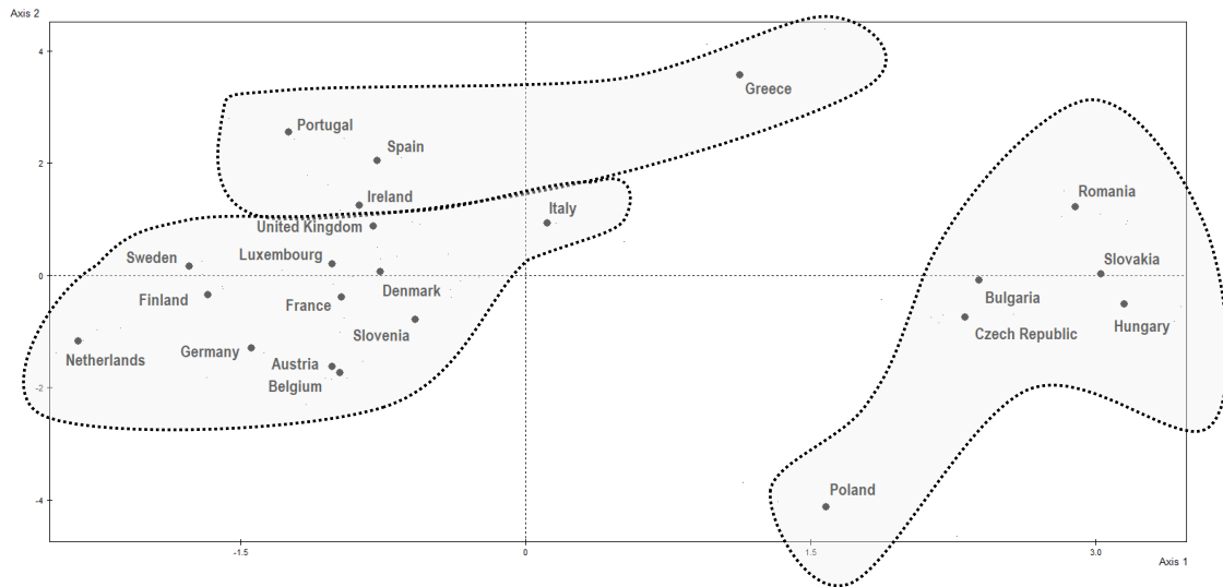
Figure 13. Clusters
