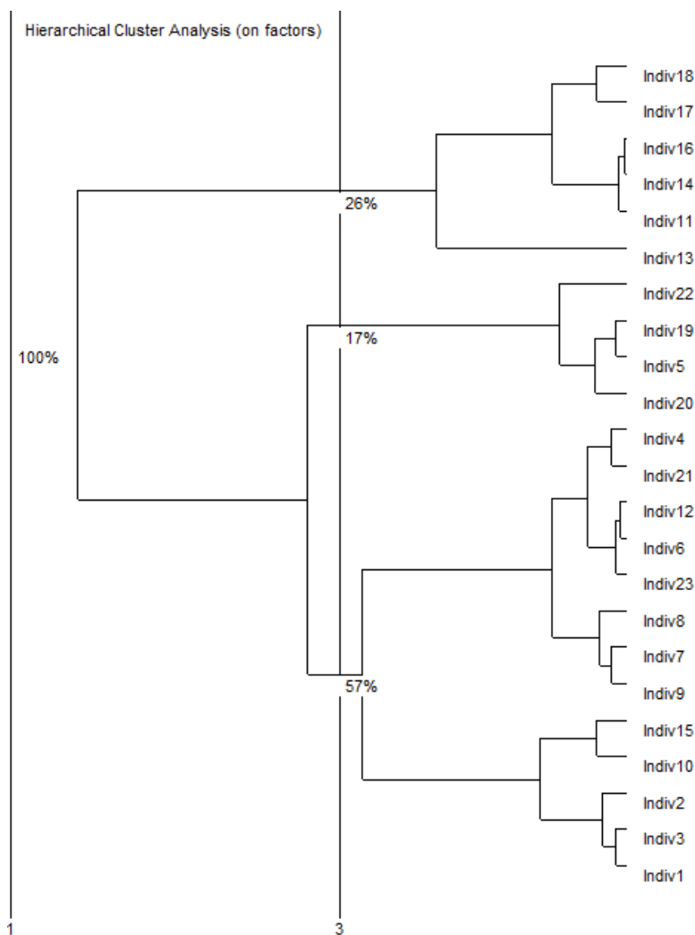
Figure 12. Dendrogram
