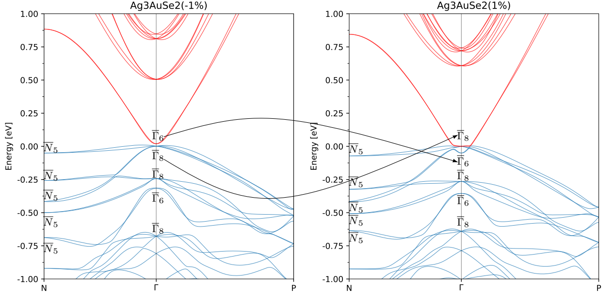
Figure 7.3: In concordance with 7.1, a band inversion is observed in this Figure. The twofold band in \Gamma above the Fermi level ( \bar{\Gamma}_6 ) in the trivial case swaps with the fourfold band ( \bar{\Gamma}_8 ).
