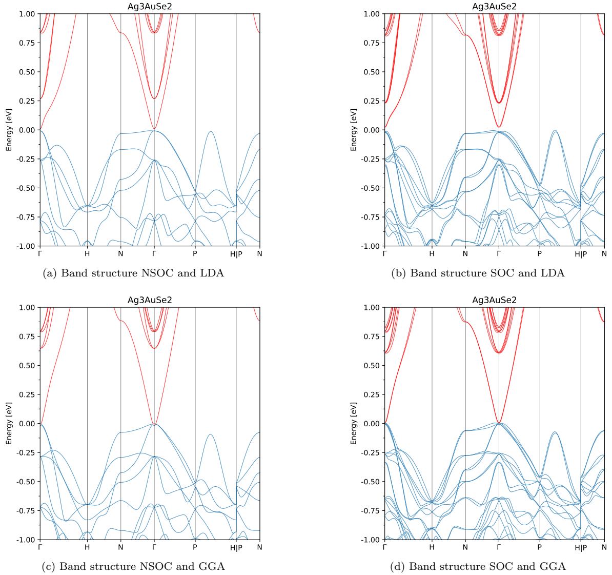
Figure 6.2: Band Structure within the range [-1eV, 1eV] having the Fermi level at the origin. The red bands represent empty (conduction) bands. The BS (c) coincides reasonably with the one Materials Project website provides, since this one is also calculated without SOC and with GGA.
