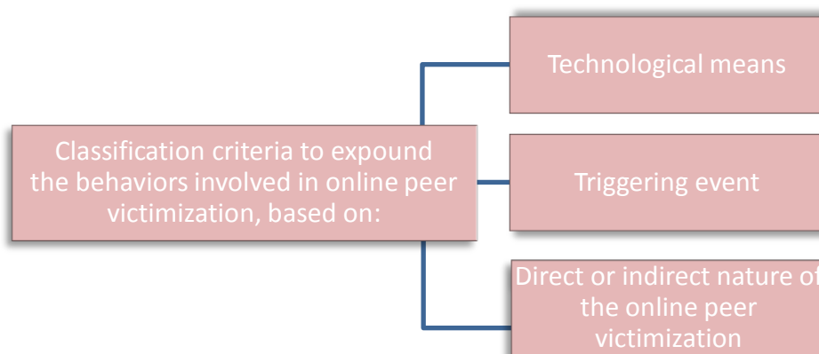
Graph 15: Classification criteria
