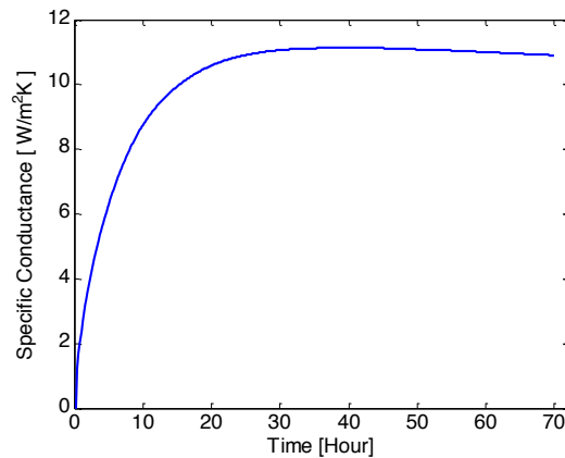
Fig. 9. Specific conductance
