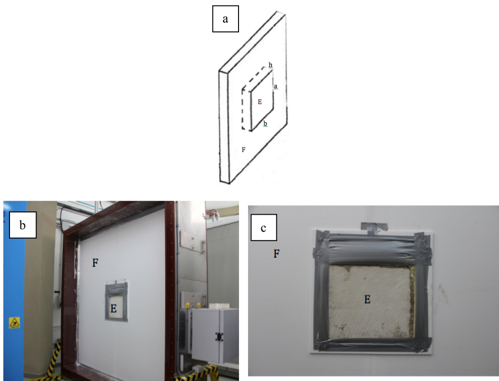
Fig. 5. The test stone (E) is contained in a frame of polyurethane . (a) Geometrical representation of the specimen, (b) Picture of the frame containing the specimen, (c) Detail of the specimen
