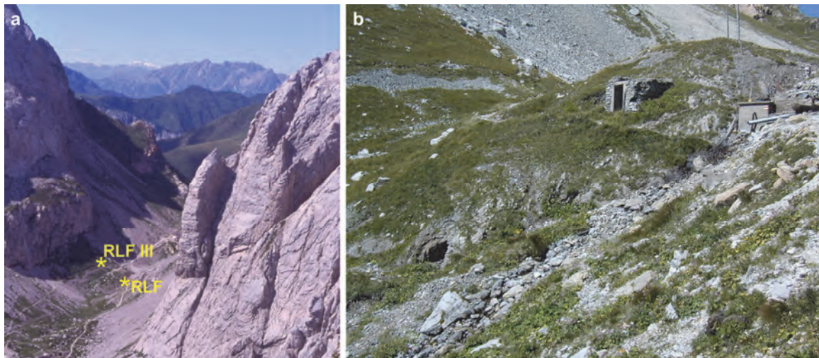
Fig. 27. a) Panoramic view of the valley south of Pass Wolayer, with location of Rifugio Lambertenghi Fontana (RFL; stop 14) and Rifugio Lambertenghi Fontana III (RLF III; stop 15) sections; b) View of the Rifugio Lambertenghi Fontana section.
