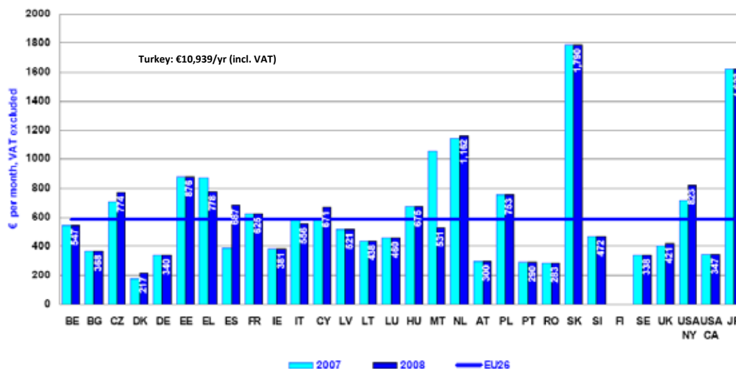
Figure 14 – Price for 2Mb/s, 2km circuits, per month
