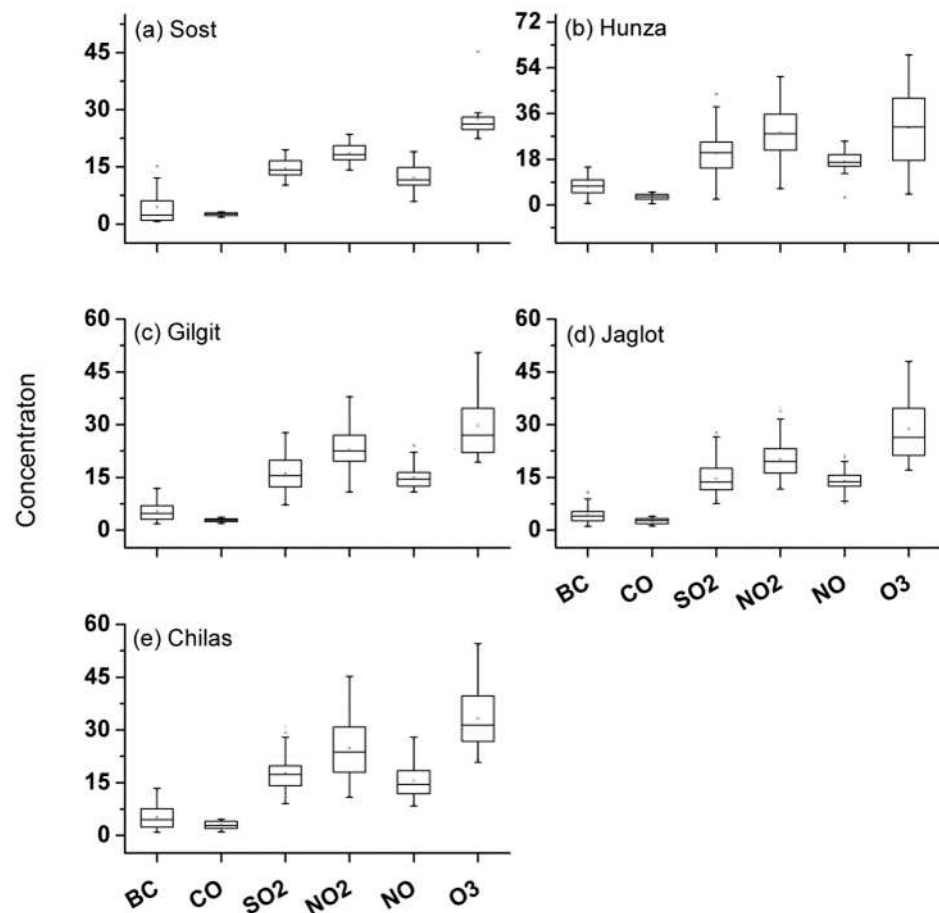
Figure 5. Variation in concentration ranges of BC ( \mu\text{g}/\text{m}^3 ), CO ( \text{mg}/\text{m}^3 ), SO 2 , NO, NO 2 and O 3 in \mu\text{g}/\text{m}^3 at selected sites in Gilgit-Baltistan during summer, 2020.
