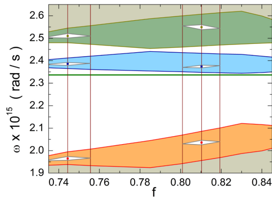
Fig. 7. Photonic band gap as a function of the fill factor, f = d_L / (d_L + d_H) . The PBG is calculated at the wave vector that corresponds to the BSW with a fixed frequency (green line). f = 0.744 and f = 0.81 for the non-optimized and optimized PhC, respectively. The white rhombic areas show variations in the photonic band edges and the light line that correspond to \pm 3\% variations in the PhC layer thicknesses (Fig. 5). The large shaded areas correspond to the thickness optimization domain. The PhC mode continuum is shown as grey areas.
