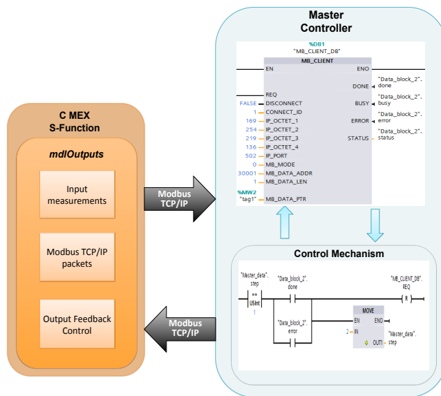
Figure 2: Communication between a simulated slave PLC and an emulated master PLC.
