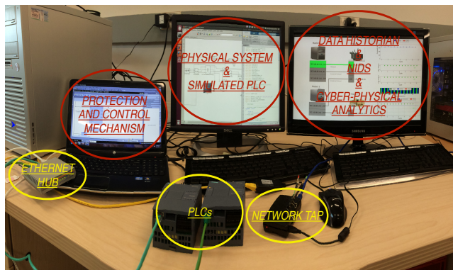
Figure 5: Deployment of our testbed environment.
