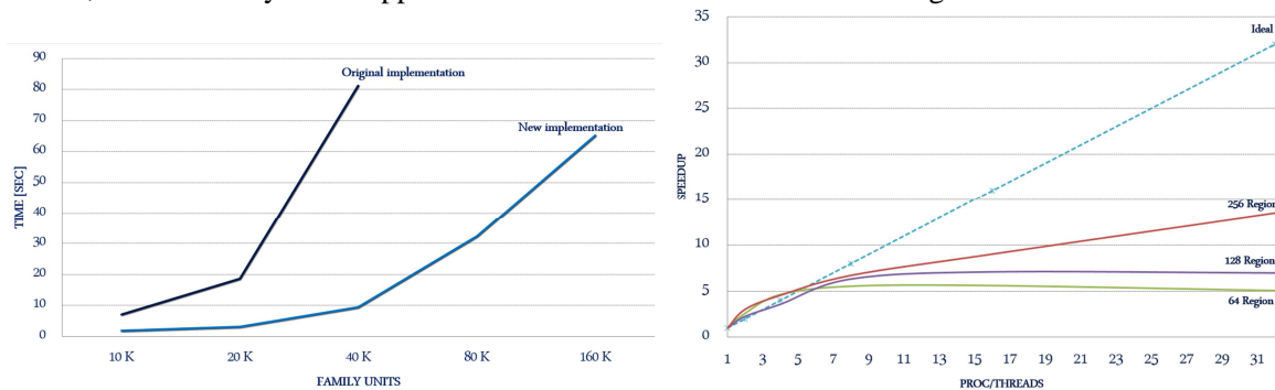
Figure 1: Comparative of Yades with previous and new implementation using ROOT-Sim in sequential (left) and parallel (right).
