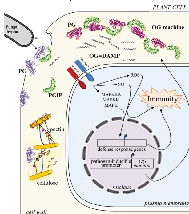
Figure 1: Schematic representation of the events occurring in the cell wall during a fungal attack of a plant tissue. Polygalacturonase (PG) secreted by the pathogen breaches the wall by degrading the pectin component. In the presence of the inhibitor PGIP degradation is slowed down and the formation of signal molecules (OG) for the activation of immunity is favoured. Expression under a pathogen-inducible promoter of a PG-PGIP fusion protein named OG-machine enhances the accumulation of OG and immunity.
