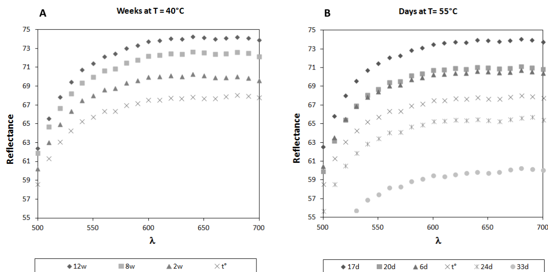
Figure 4. Colorimetric analysis: reflectance spectra of infant milk formulas stored up to 12 weeks at 40 °C (A) or up to 33 days at 55 °C (B).
