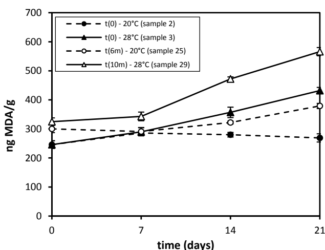
Figure 3. Nanograms of MDA found in 1 g of infant milk formula stored for three weeks, after opening, at 20 or 28 °C. Samples 2 and 3 were analyzed just after manufacturing, whereas Samples 25 and 29 were opened after 6 or 10 months of storage at 20 °C, respectively.
