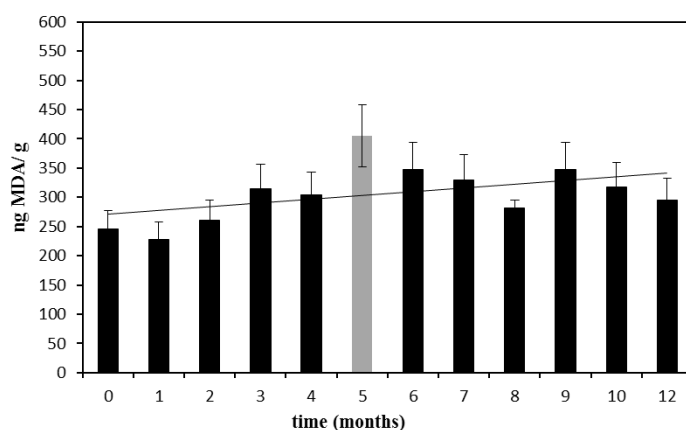
Figure 2. Nanograms of MDA found in 1 g of infant milk formula stored at 20 °C sealed in the original package. The trend-line was calculated excluding the outlier point at the fifth month. Error bars are the %RSD.
