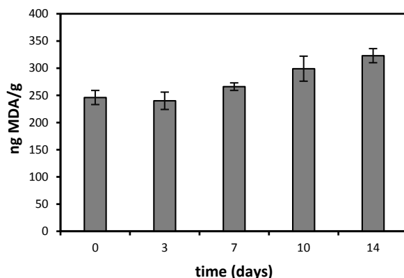
Figure 1. Nanograms of malondialdehyde (MDA) found in 1 g of infant milk formula stored at 55 °C sealed in the original package. Error bars are relative standard deviation (%RSD).
