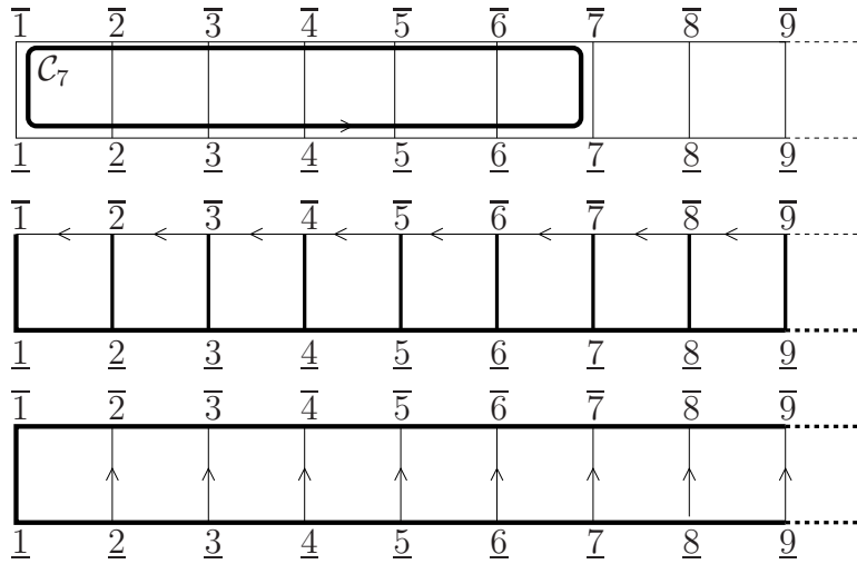
FIGURE 2. Top. The graph G is the ladder with vertex set \{\underline{1}, \underline{2}, \dots\} \cup \{\overline{1}, \overline{2}, \dots\} , cycle \mathcal{C}_n is given by (\underline{1}, \underline{2}, \dots, \underline{n}, \overline{n}, \overline{n-1}, \dots, \overline{1}) . Center. The fundamental tree \mathcal{T}^{(1)} is the bold comb. The arrows correspond to the chords. The basis cycle \mathcal{C}_k^{(1)} is given by (\overline{k+1}, \overline{k}, \underline{k}, \underline{k+1}) . Bottom. The fundamental tree \mathcal{T}^{(2)} is in boldface. The basis cycle \mathcal{C}_k^{(2)} equals \mathcal{C}_k .
