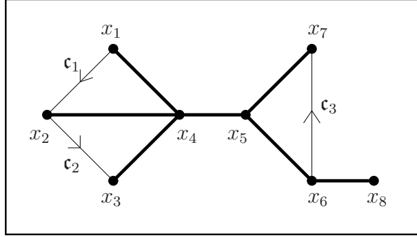
FIGURE 1. Fundamental basis. The bold edges form the spanning tree \mathcal{T} . The chords c_1 = (x_1, x_2) , c_2 = (x_2, x_3) and c_3 = (x_6, x_7) correspond to the cycles \mathcal{C}_{c_1} = (x_1, x_2, x_4) , \mathcal{C}_{c_2} = (x_2, x_3, x_4) and \mathcal{C}_{c_3} = (x_6, x_7, x_5) , respectively.
