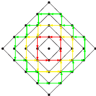
FIGURE 3. The vector field F when U = \tilde{U}(|x|_1)
