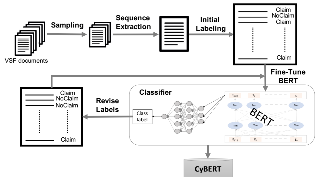
Figure 2. Overview of CyBERT workflow.
