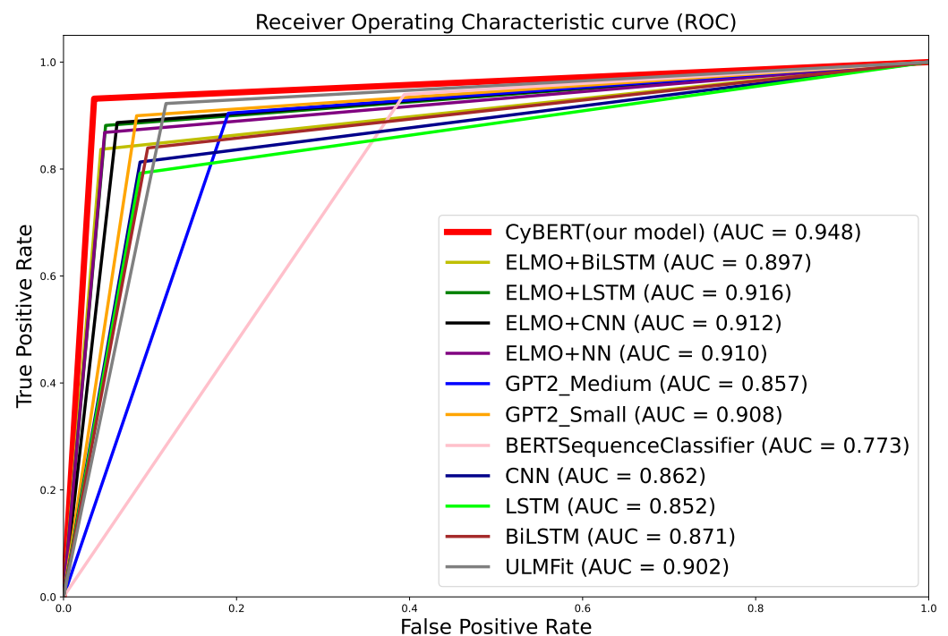
Figure 11. ROC comparison for all models.
