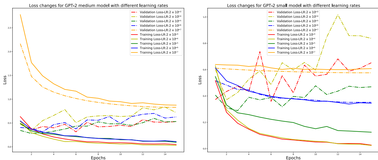
Figure 9. Loss changes for GPT-2 models with different learning rates: GPT-2 medium (left) and GPT-2 small (right) for 15 epochs.
