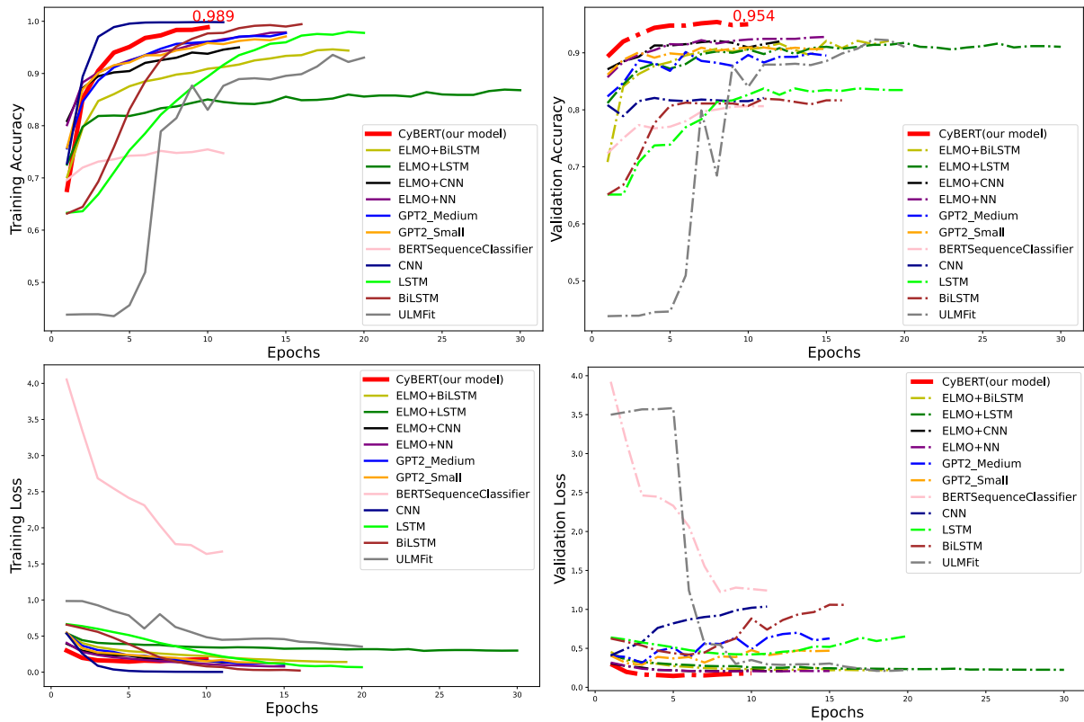
Figure 10. Comparing training accuracy (left top), validation accuracy (right top), training Loss (bottom left), and validation loss (bottom right) for all models.
