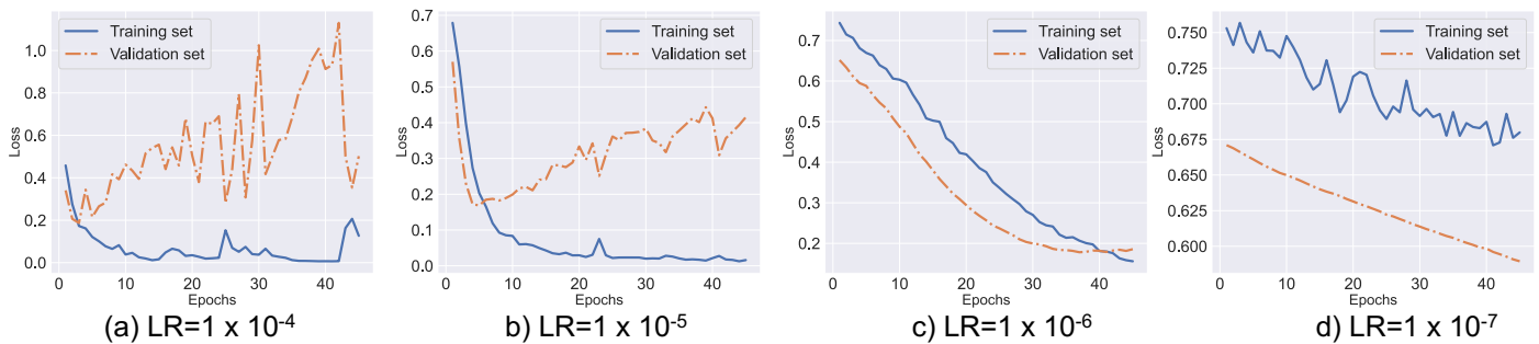
Figure 4. Learning rate effect on model convergence.
