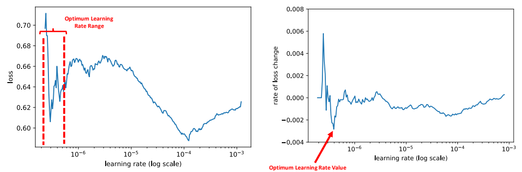
Figure 5. Impact of learning rates when fine-tuning our model.
