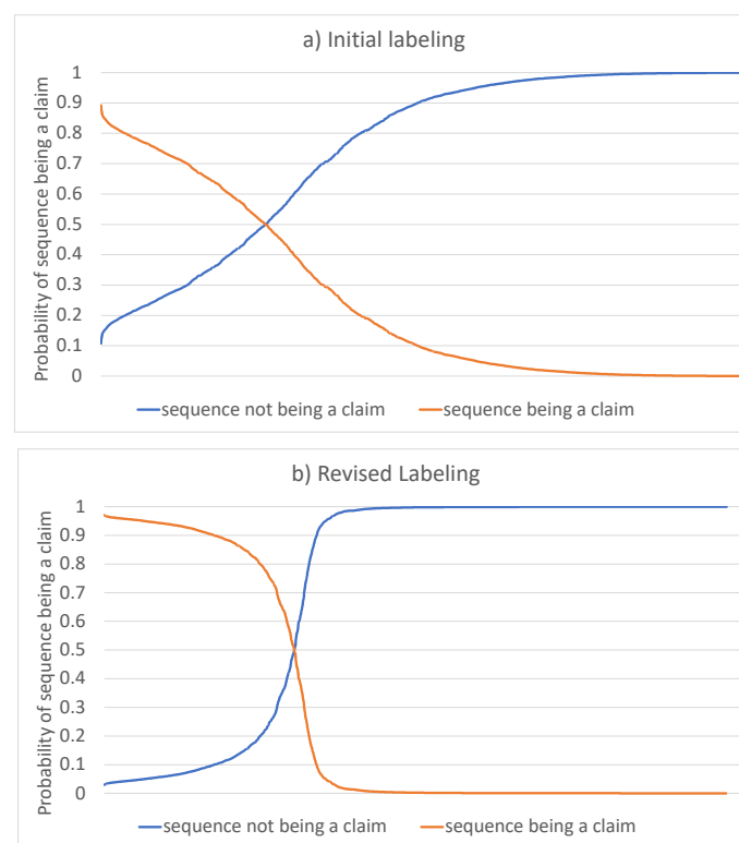
Figure 7. Sorted probabilities with (a) initial labeling and (b) revised labeling.
