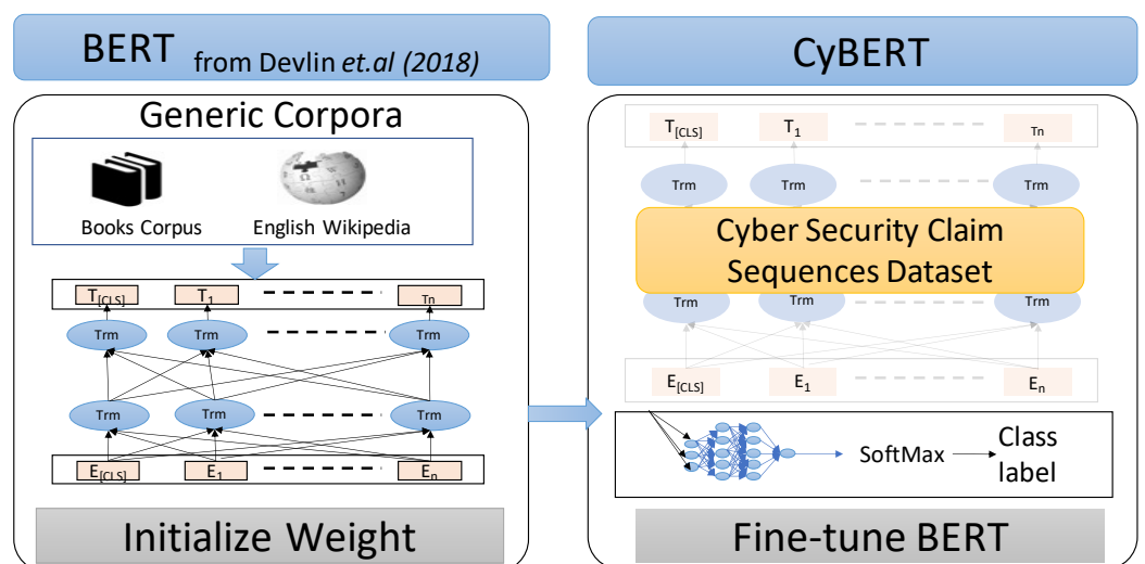
Figure 3. Overview of fine-tuning BERT for CyBERT.
