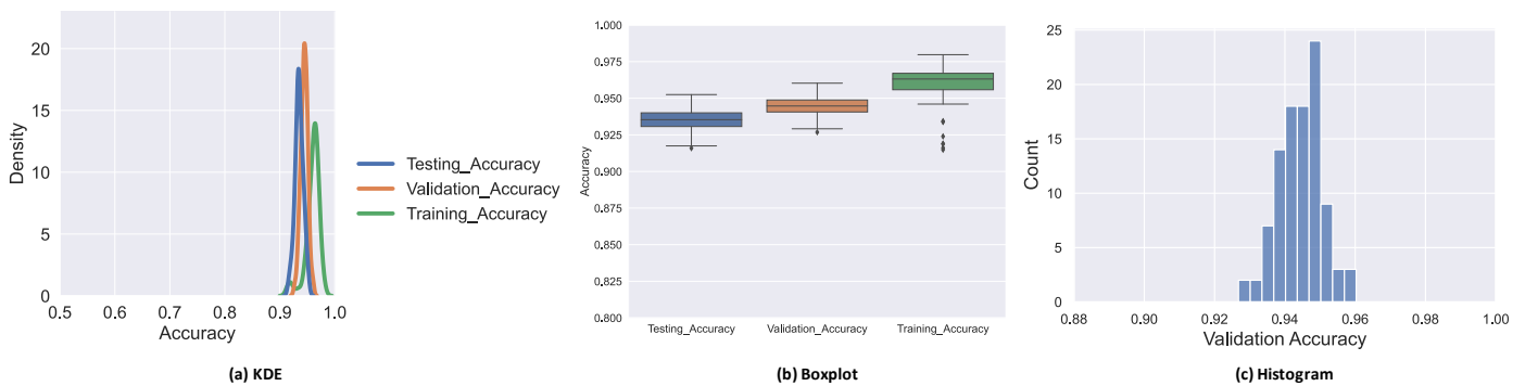
Figure 8. Kernel density estimation (a); box plot (b) for training, validation, and testing accuracy; validation accuracy histogram (c).
