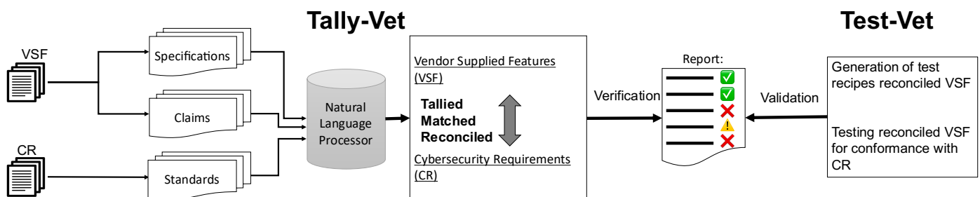
Figure 1. Overall workflow of the CYVET cybersecurity vetting approach.
