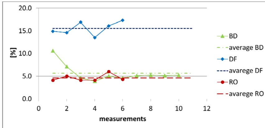
Figure 5. Exhaust opacity.
