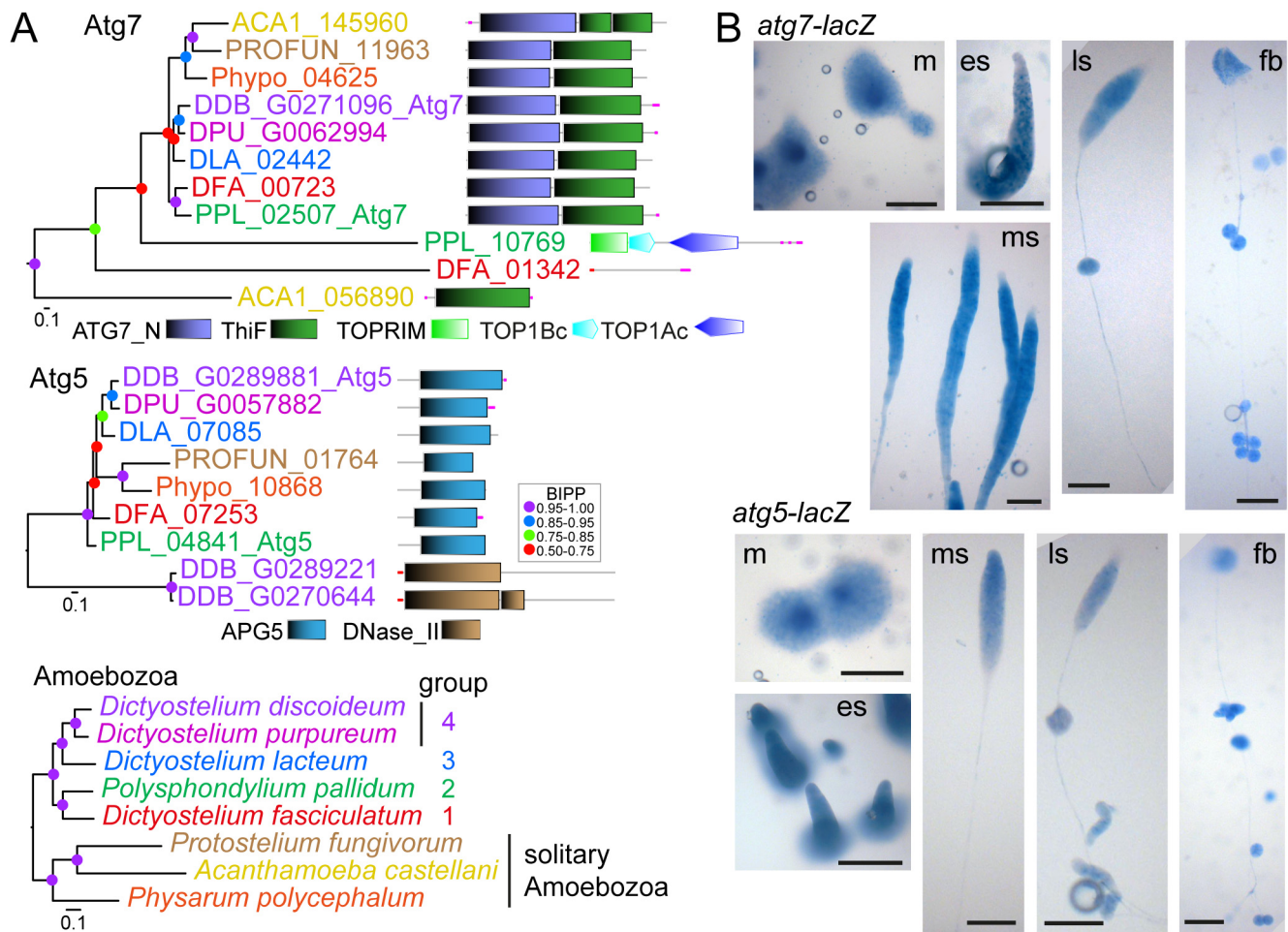
Figure 2. Identification and expression patterns of P. pallidum strain PN500_J ( Ppal ) atg7 and atg5 . A. Identification. The previously identified Dictyostelium discoideum ( Ddis ) atg7 and atg5 genes (Otto et al. , 2003) were used as bait to identify homologs in well-annotated dictyostelid and solitary amoebazoan genomes. Protein sequences of all hits were aligned with the Ddis sequences and the alignment was used to infer phylogenies using MrBayes 3.2 (Ronquist & Huelsenbeck, 2003). Posterior probabilities of the nodes (BIPP) are indicated by coloured dots. Trees were annotated with the functional domain architecture of the proteins as analysed with SMART (Schultz et al. , 1998). A multigene amoebazoan phylogeny (Schilde et al. , 2019) is shown as reference. B. Expression. Ppal cells, transformed with gene fusions of the Ppal atg7 or atg5 promoters and Escherichia coli lacZ , were plated on nitrocellulose filters supported by non-nutrient (NN) agar. Developing structures were fixed in glutaraldehyde and stained with X-gal (Dingermann et al. , 1989). m: mound; es, ms and ls: early, mid- and late sorogens; fb: fruiting body. Bar: 100 μm.
