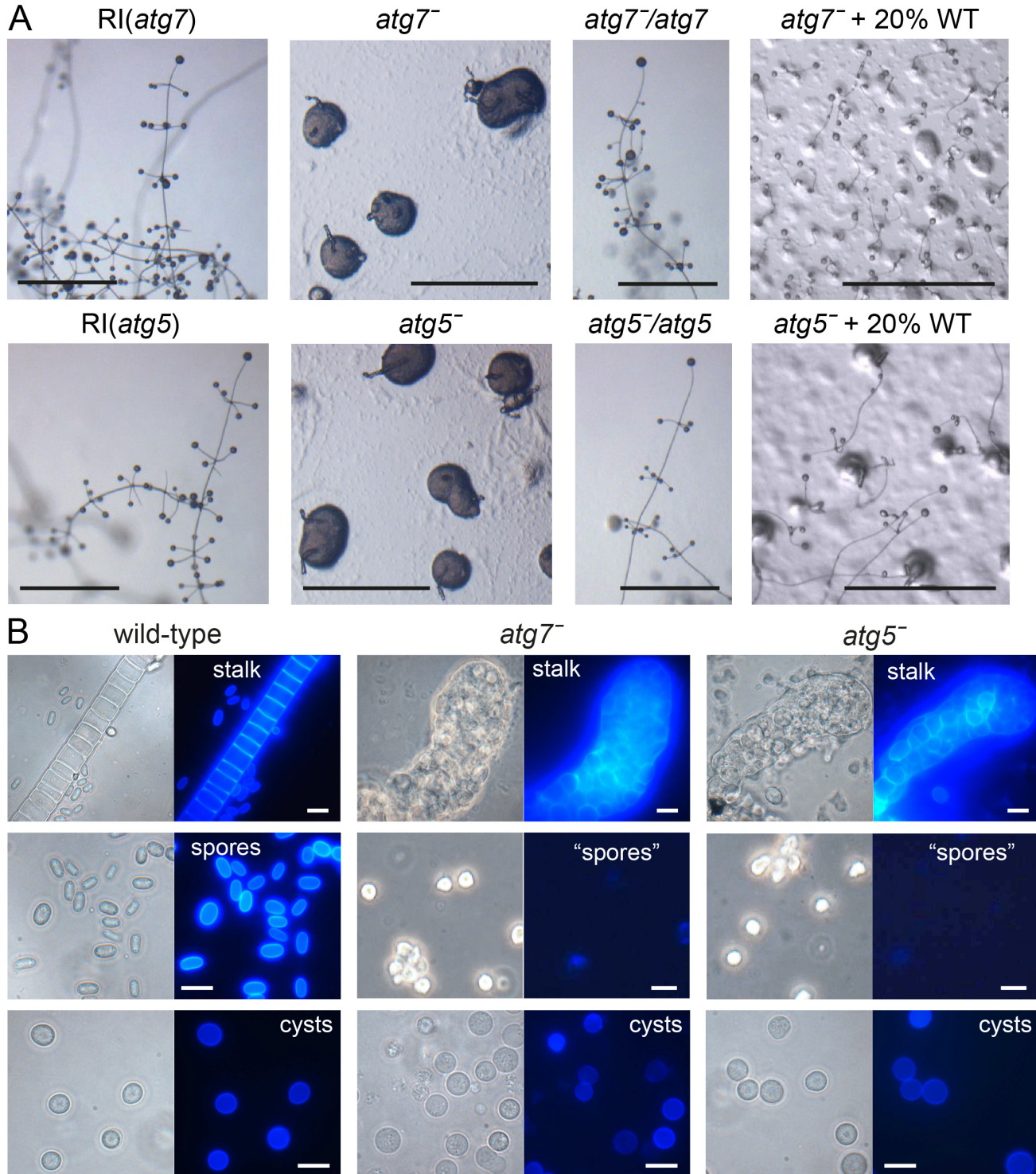
Figure 3. Phenotypes of P. pallidum strain PN500_J ( Ppal ) atg7 and atg5 mutants. A. Ppal atg7 - and atg5 - knock-outs, random integrant (RI) and atg7 - and atg5 - cells complemented with atg7 or atg5 , respectively, or mixed with 20% wild-type (WT) were plated on non-nutrient (NN) agar and incubated until mature terminal structures had formed. Bar: 100 \mu m. B. Terminal structures of WT, atg7 - and atg5 - were directly transferred to 0.001% Calcofluor on a slide glass, or for atg7 - and atg5 - structures also first dissociated in 0.001% Calcofluor by vigorous pipetting and then transferred. Stalks, spores and cysts were photographed under phase contrast (left panels) and UV (right panels). Bar: 10 \mu m.
