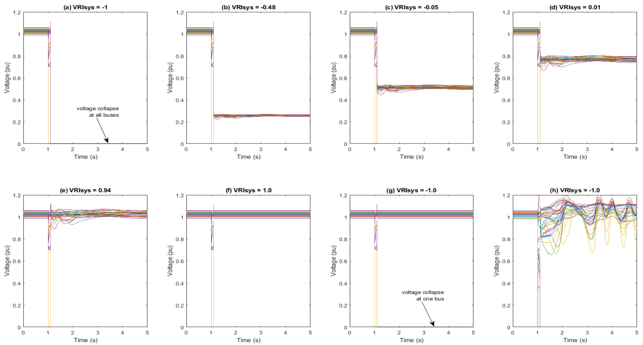
FIGURE 12. Different voltage waveforms showing different VRI_{sys} .
