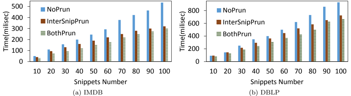
Figure 9: Snippet processing efficiency in one step.
