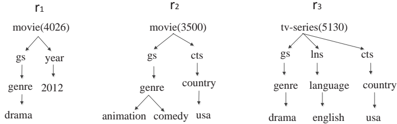
Figure 3: XML subtree snippets
