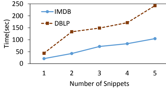
Figure 11: Naive method without using index
