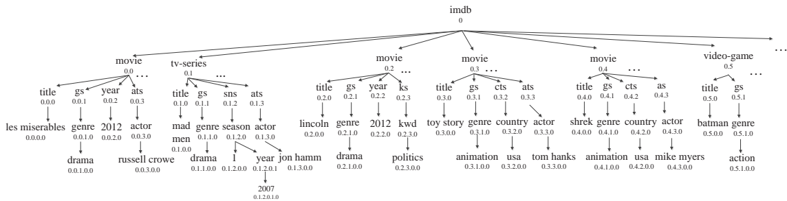
Figure 1: A part of IMDB dataset
