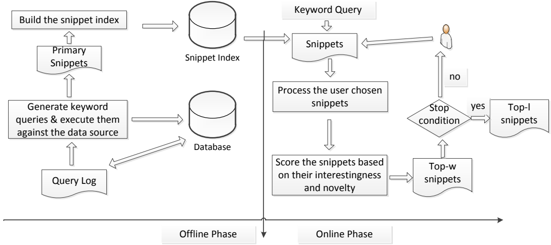
Figure 4: XSnapshots architecture overview
