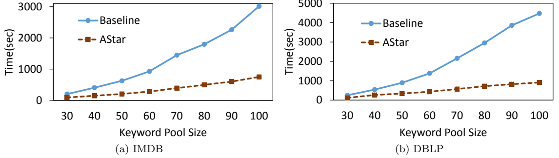
Figure 7: Keyword pool size |\mathcal{K}| effect on the efficiency of computing primary snippets.
