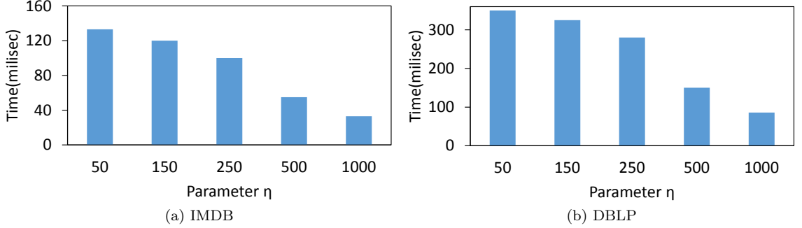
Figure 10: The effect of parameter \eta on the efficiency.
