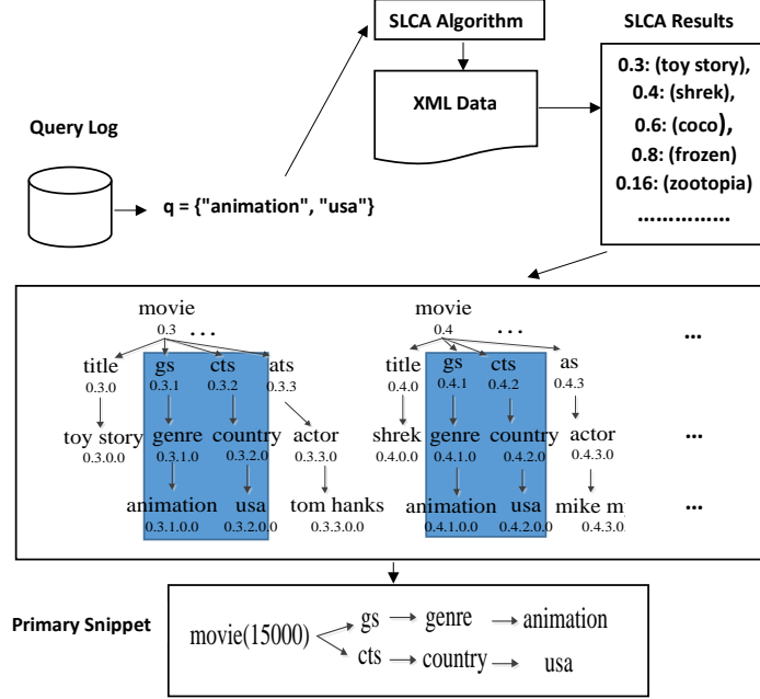
Figure 2: Primary snippet generation
