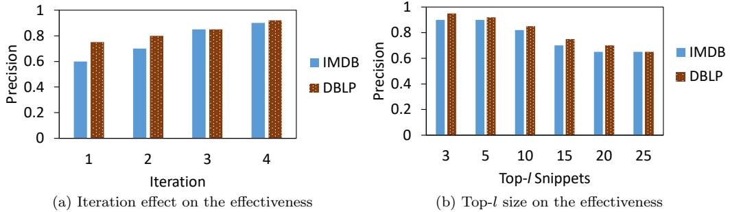
Figure 6: Quality of Top- l snippets.
