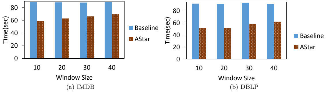
Figure 8: Window size w effect on the efficiency of computing primary snippets.
