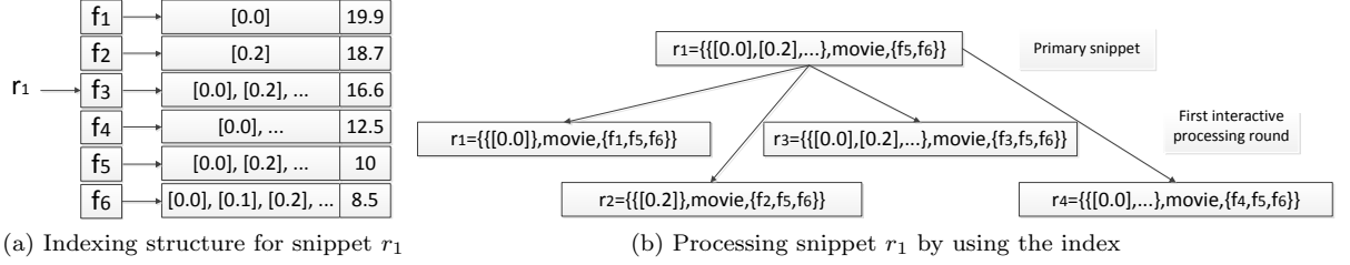
Figure 5: Snippet processing by using indexing structure.
