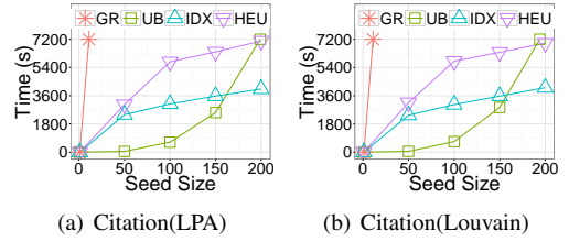
Figure 7: Efficiency of proposed algorithms in DBLP dataset
