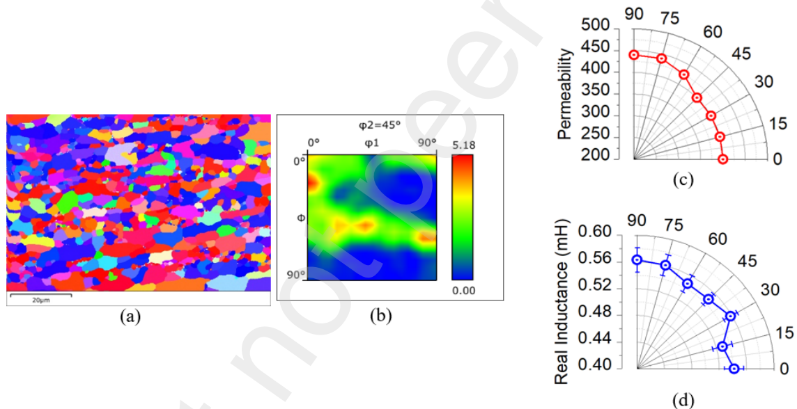
Figure 8. Inverse pole figure (IPF) map (a), ODF map (b) predicted magnetic permeability using the texture model (c) and the angular dependence of inductance at a series of angles from 0^\circ , 15^\circ , 30^\circ , 45^\circ , 60^\circ , 75^\circ and 90^\circ with respect to the RD (d) in the packaging steel sample.
