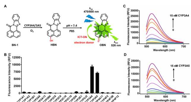
Figure 1. Fluorescence response of BN-1 toward CYP3A. A) Proposed mechanism of CYP3A triggering the fluorescence response of BN-1 . B) Fluorescence response of BN-1 following incubation with various human CYPs. Data are shown as the mean \pm S.D. ( n = 3 ). Fluorescence spectra of BN-1 following incubation with increasing concentrations of CYP3A4 (C) and CYP3A5 (D).
