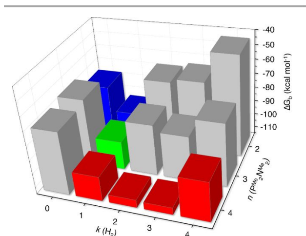
Figure 6 Speciation free energy landscape of [\text{Nb}_2(\text{CH}_3\text{CN})_m(\text{PMe}_2\text{NMe}_2)_n(\text{H}_2)_k]^{4+} . Gray bars indicate high energy species, while the colored bars show intermediates involved in the lowest free energy pathway from 2 ( n = 2, m = 4, k = 0 ) to 4.H 8 ( n = 4, m = 0, k = 4 ). Blue: species with n = 2 ; green: species with n = 3 ; red: species with n = 4 . Energies were obtained at the B3LYP-D3(BJ)/def2-TZVPP+PCM level following eq. 1.
