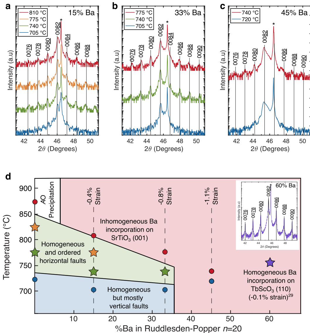
FIG. 4. (a)–(c) XRD \theta - 2\theta scans for a series of (\text{ATiO}_3)_{20}\text{AO} films grown at different temperatures with barium concentrations of 15%, 33%, and 45%, respectively, on \text{SrTiO}_3 (001) substrates. (d) Diagram summarizing the optimal growth conditions for the growth of (\text{ATiO}_3)_{20}\text{AO} films on \text{SrTiO}_3 (001) substrates as a function of barium content and substrate temperature. The color of each data point corresponds to the color of the film's XRD spectrum in Figs. 2(b) and 4(a)–4(c). Starred data points indicate conditions for which the highest quality films were synthesized, and the region shaded green indicates the "growth window" in which high quality films can be synthesized on \text{SrTiO}_3 (001) substrates. The purple star outside the growth window marks the growth conditions with which a high quality (\text{ATiO}_3)_{20}\text{AO} film was grown on a \text{TbScO}_3 (110) substrate (from Ref. 29), and the inset shows the corresponding XRD \theta - 2\theta scan of the previously reported film.
