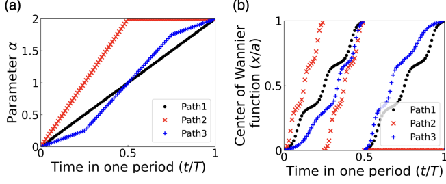
FIG. 3. Deformation of the parametric paths with the same Chern number on the t - k space. (a) Three paths with the same initial value \alpha(t=0) = 0 and the same final value \alpha(t=T) = 2 within one period. (b) The evolution of the center of the Wannier function for each path within one period.
