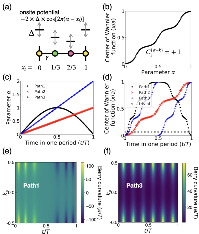
FIG. 2. Bulk 1D periodic three-site tight-binding model with a non-trivial quantum pumping. (a) The unit cell with the parameters described in the main text. (b) The evolution of the center of the Wannier function for the lowest band (labelled by 1) along a loop of the parametric variable \alpha . The Chern number on the \alpha - k plane, C_1^{\{\alpha-k\}} , is 1. (c) Three chosen paths for \alpha(t) . Path1: \alpha(t) = \sin^2(\pi t/T) ; Path2: \alpha(t) = t/T ; Path3: \alpha(t) = 2t/T . (d) The evolution of the center of the Wannier function for each path within one period. For comparison, we provide a trivial case [see Eq. (3)], of which the Wannier function remains a constant, in this case, 0.07. (e) and (f) The Berry curvature on the t - k plane for Path1 ( C_1^{\{t-k\}} = 0 ) and Path3 ( C_1^{\{t-k\}} = 2 ), respectively.
