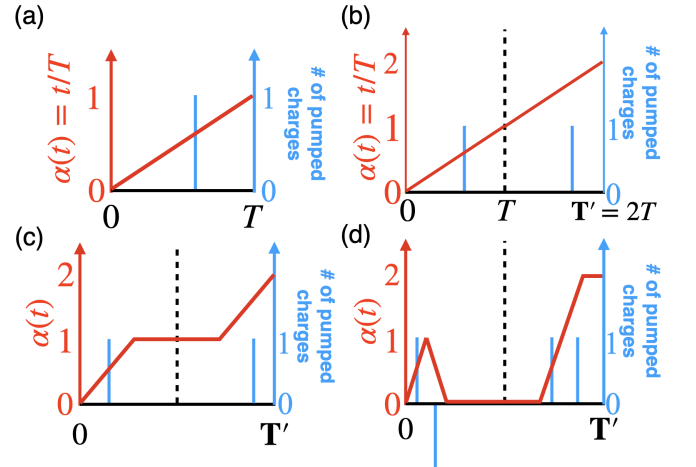
FIG. 1. Schematic illustration of the formula C_n^{\{t-k\}} = l C_n^{\{\alpha-k\}} . (a) The path for the parametric variable \alpha(t) = t/T where T is the period. (b) The extension of (a) with a newly defined period T' = 2T . (c) and (d) Two deformed parametric paths and the corresponding number of pumped charges as a function of time within the new time period T' .
