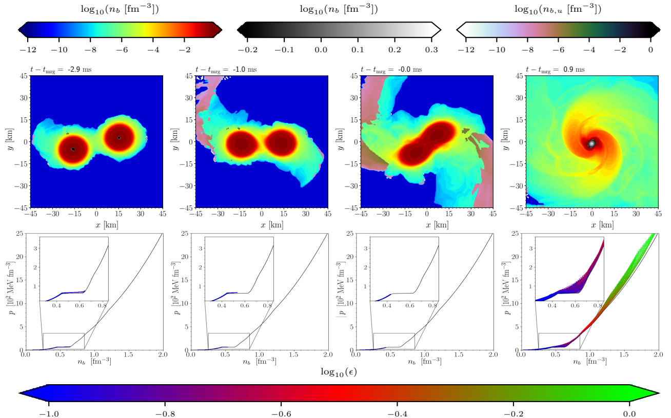
FIG. 3. Snapshots of the baryon number density in the equatorial plane (upper panels) and the respective baryon number density-pressure phase diagram (lower panels) for the PT1 case employing the highest resolution. We represent the hadronic matter density in the upper left colorbar, the quark matter density in upper middle colorbar and the ejecta density in the upper right colorbar. The lower colorbar refers to the specific internal energy. Upper panels, first column : at this instance, the inner core contains quarks at \log_{10}(n_b [\text{fm}^{-3}]) \sim -0.1 . Upper panels, second column : the stars are tidally deformed, decreasing the core densities. The inner cores no longer contain quarks, since they reach maximum densities of \log_{10}(n_b [\text{fm}^{-3}]) \sim -0.3 , below the threshold value at which quarks are present. Upper panels, third column : moment of merger, where we remark the complete absence of quarks in the coalescing material. Upper panels, fourth column : in less than 1 ms after the merger, a sizeable quark-matter core is formed, which then quickly collapses to a BH. Lower panels : The zero-temperature PT1 EOS is depicted (black line) along with the color-coded specific internal energies for the respective snapshots; from this plot it is clear that at late stages of the inspiral, the quarks in the core of both stars vanish, marking “the reverse phase transition”.
