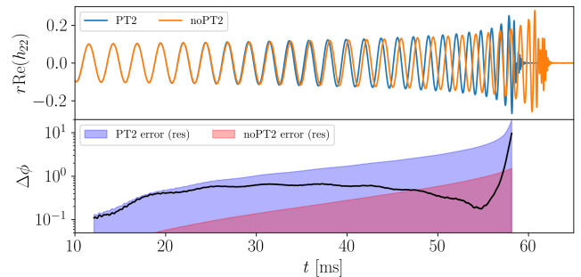
FIG. 6. Top panel: (2,2)-mode of the highest resolution waveform for PT2 (blue) and noPT2 (orange) scenarios. Bottom panel: The black line shows the GW phase difference between the Richardson extrapolated waveform for PT2 and noPT2. Shaded areas show the error on the GW \phi for each system computed with Eq. (A1). In contrast to Fig. 4 we do not incorporate an additional phase difference based on simulations with different ID resolutions.
