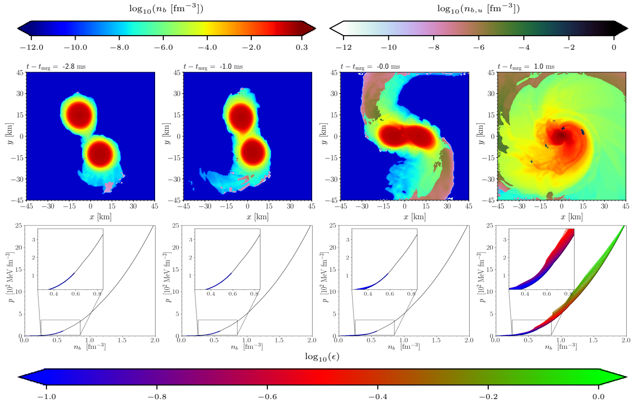
FIG. 7. Snapshots of the baryon number density on the equatorial plane (upper panels) and the respective baryon number density-pressure phase diagram (lower panels), together with the zero-temperature EOS (black line) and color-coded specific internal energy, are depicted for the noPT2 setup employing the highest resolution. Hadronic matter is represented by the upper left colorbar and matter identified as ejecta by the upper right colorbar.
