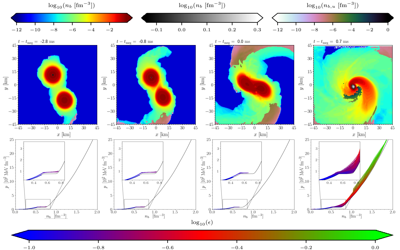
FIG. 8. Snapshots of the baryon number density on the equatorial plane (upper panels) and the respective baryon number density-pressure phase diagram (lower panels) for the PT2 case are depicted employing the highest resolution. Similarly to Fig. 3, we represent hadronic matter in the upper left colorbar, the quark matter using the upper middle colorbar and the ejecta using the colorbar on the upper right. The lower colorbar refers to the specific internal energy. Upper panels, first column: at this instance we notice that the inner core of one of the stars contains quarks at \log_{10}(n_b [\text{fm}^{-3}]) \sim -0.1 . Upper panels, second column: the densest portions of the stars are found tidally deformed. The inner core containing quarks is smaller and less dense with \log_{10}(n_b [\text{fm}^{-3}]) < -0.1 . Upper panels, third column: moment of merger, where we note the complete absence of quarks in the coalescing material. Upper panels, fourth column: in less than 1 ms after the merger a sizeable quark-matter core is formed, which then quickly collapses to a BH. Lower panels: The zero-temperature PT2 EOS is depicted (black line) along with the color-coded specific internal energies for the respective snapshots; similarly to the PT1 case, we see the decrease of the quarks content within the star towards the merger and its subsequent increase rapidly after the merger.
