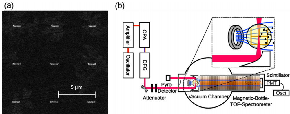
FIG. 1. (a) Scanning electron micrograph of a nanorod array (rod length 1 \mu\text{m} ). (b) Experimental setup. Tunable mid-infrared pulses are focused onto a nanorod array in a high vacuum chamber. Electron kinetic energy spectra are measured with a magnetic-bottle time-of-flight spectrometer.
