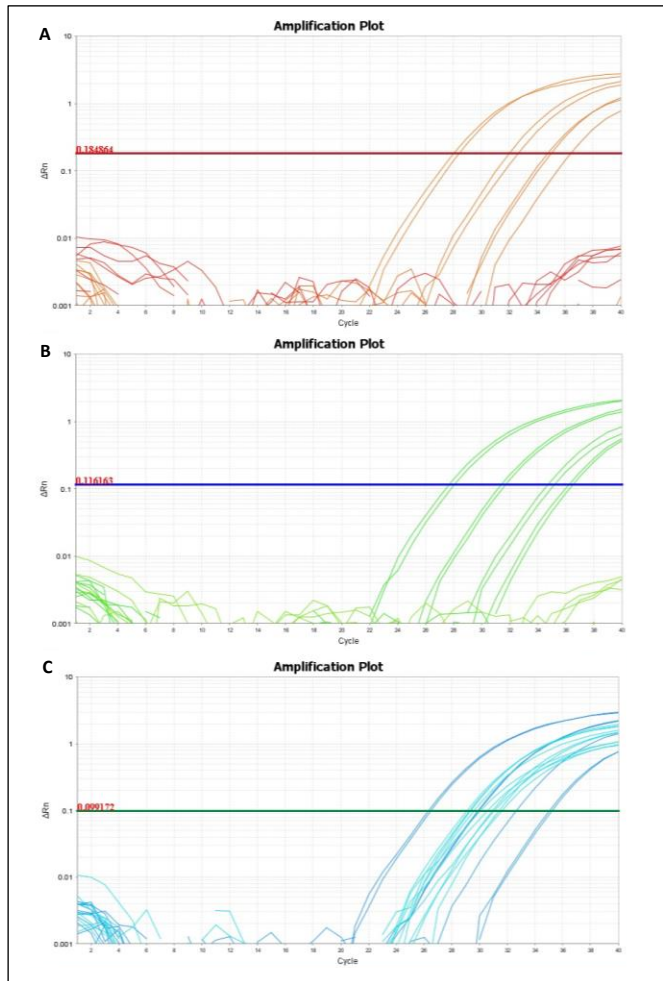
Figure 3. QPCR test for detection of COVID-19 RNA. (A) COVID-19 N1 assay, (B) COVID-19 N2 assay, (C) Human RNase-P Control Assay. Amplification curves in all assays demonstrated expected performance of the assays in the standard curve samples. Amplification curves in all samples in panel C (For the human RNase-P gene) demonstrate the amplification-suitable quality of the RNA extracted.
