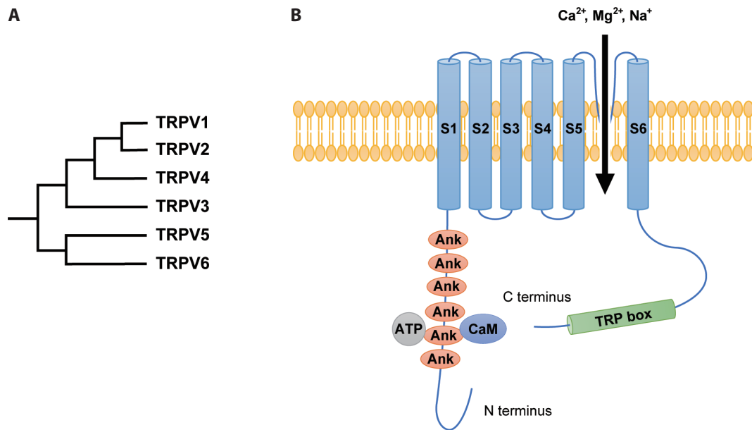
Figure 1. Phylogenetic tree (A) and common structure (B) of TRPV family. Structurally, TRPV family has two domains. S1–S4 voltage-sensing domains associates with the transmembrane segments S5–S6 containing the pore region. TRPV1 is a tetramer, and its pore-like structure comprises the large basket-shaped cytoplasmic and transmembrane regions. TRPV family has six ankyrin (Ank) repeat domains at their N-termini. Ank repeat of TRPV1 has an ATP-binding site and a calmodulin (CaM)-binding site, important for channel activation and inactivation, respectively. TRP-box in the C-terminal region is important for activating channel gating and protein tetramerization.
