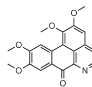
Oxoglucine
