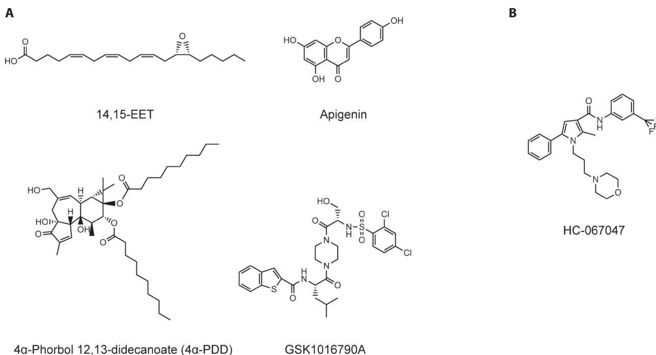
Figure 5. Chemical structures of TRPV4 agonists (A) and antagonist (B).
