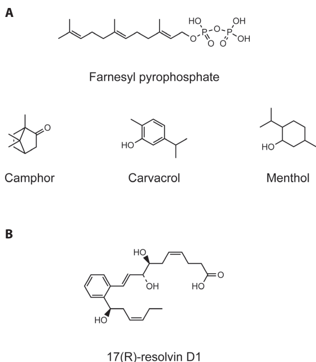
Figure 4. Chemical structures of TRPV3 agonists (A) and antagonist (B).
