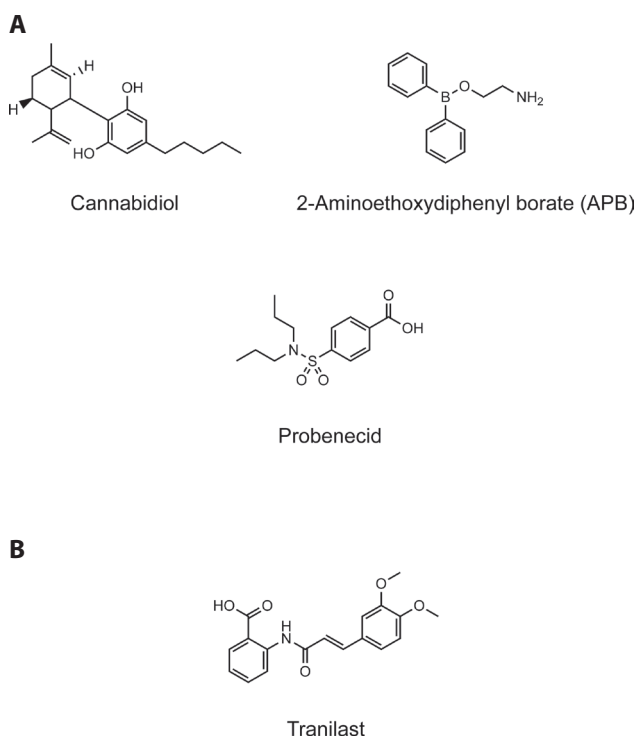
Figure 3. Chemical structures of TRPV2 agonists (A) and antagonist (B).
