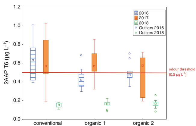
Figure 4. Box plots of distribution of 2-aminoacetophenone (2AAP) in wines obtained from grapes cultivated using different agronomic systems after accelerated ageing ( 40 \text{ }^\circ\text{C} , 6 days); concentrations are reported in \mu\text{g L}^{-1} .
