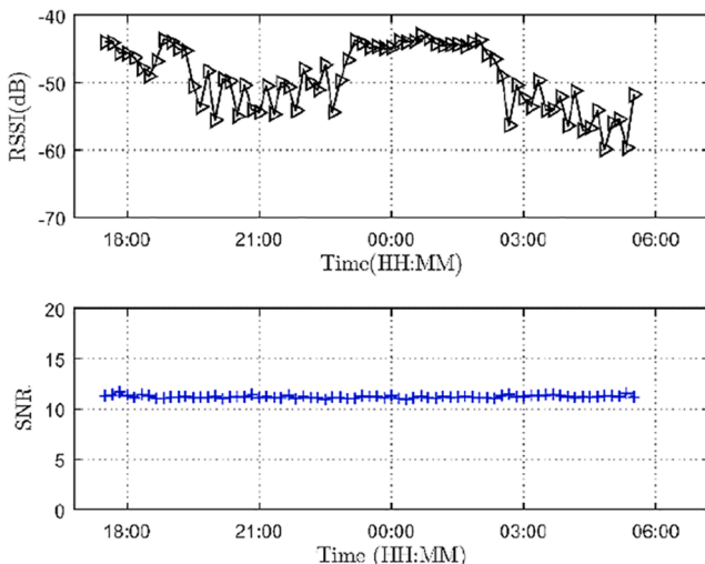
Fig. 19. LoRa signal characteristics as a function of time: RSSI and SNR.
