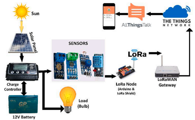
Fig. 3. System architecture of the smart energy meter.
