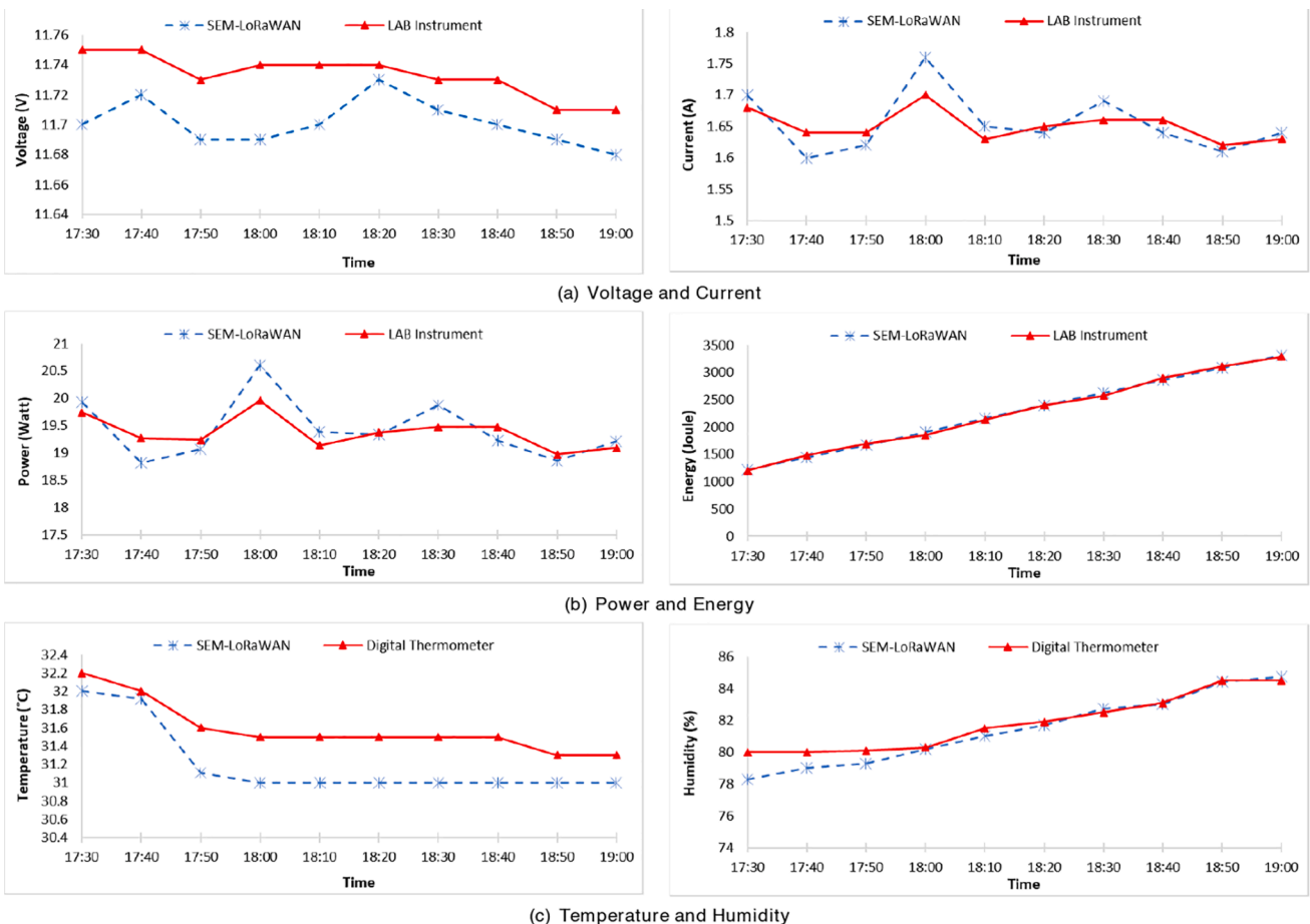
Fig. 22. Comparison of SEM-LoRaWAN and LAB instrumentation measurements.
