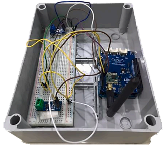
Fig. 8. System testing box on breadboard.
