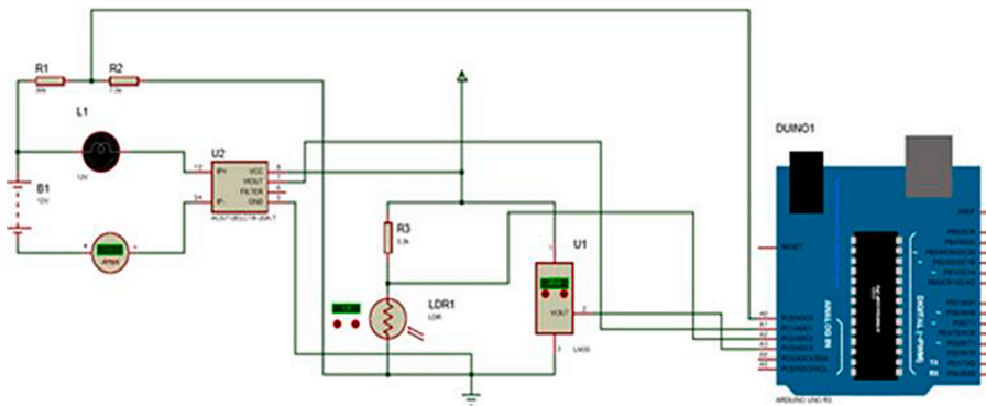
Fig. 5. Circuit simulation using Proteus.
