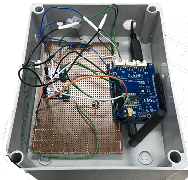
Fig. 11. LoRa node connections on donut board.
