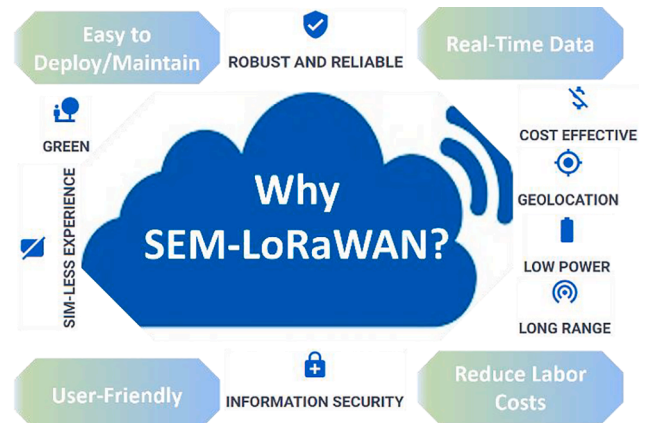
Fig. 1. Research motivations.
