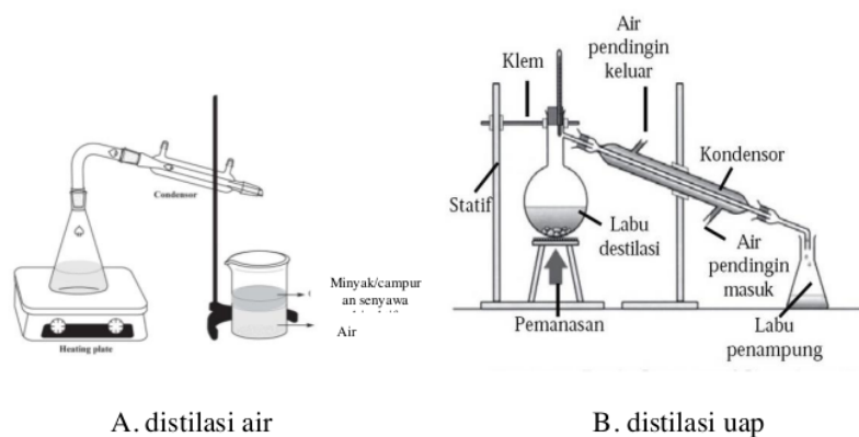
Gambar 5.9. Distilator: Distilasi air (A) dan distilasi uap (B) (Suleria and Barrow, 2020).
