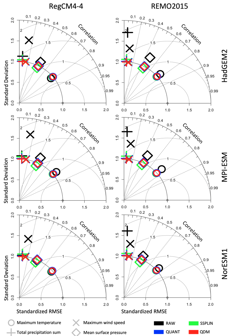
Figure 2. Taylor diagrams to evaluate the performance of three bias adjustment methods. The underlying GCM and RCM of each of the six model combinations is given in the row label and column label, respectively. The four variables are distinguished by symbols, the bias adjustment methods by colors. Taylor diagrams consist of correlation, normalized RMSE and normalized standard deviation.
