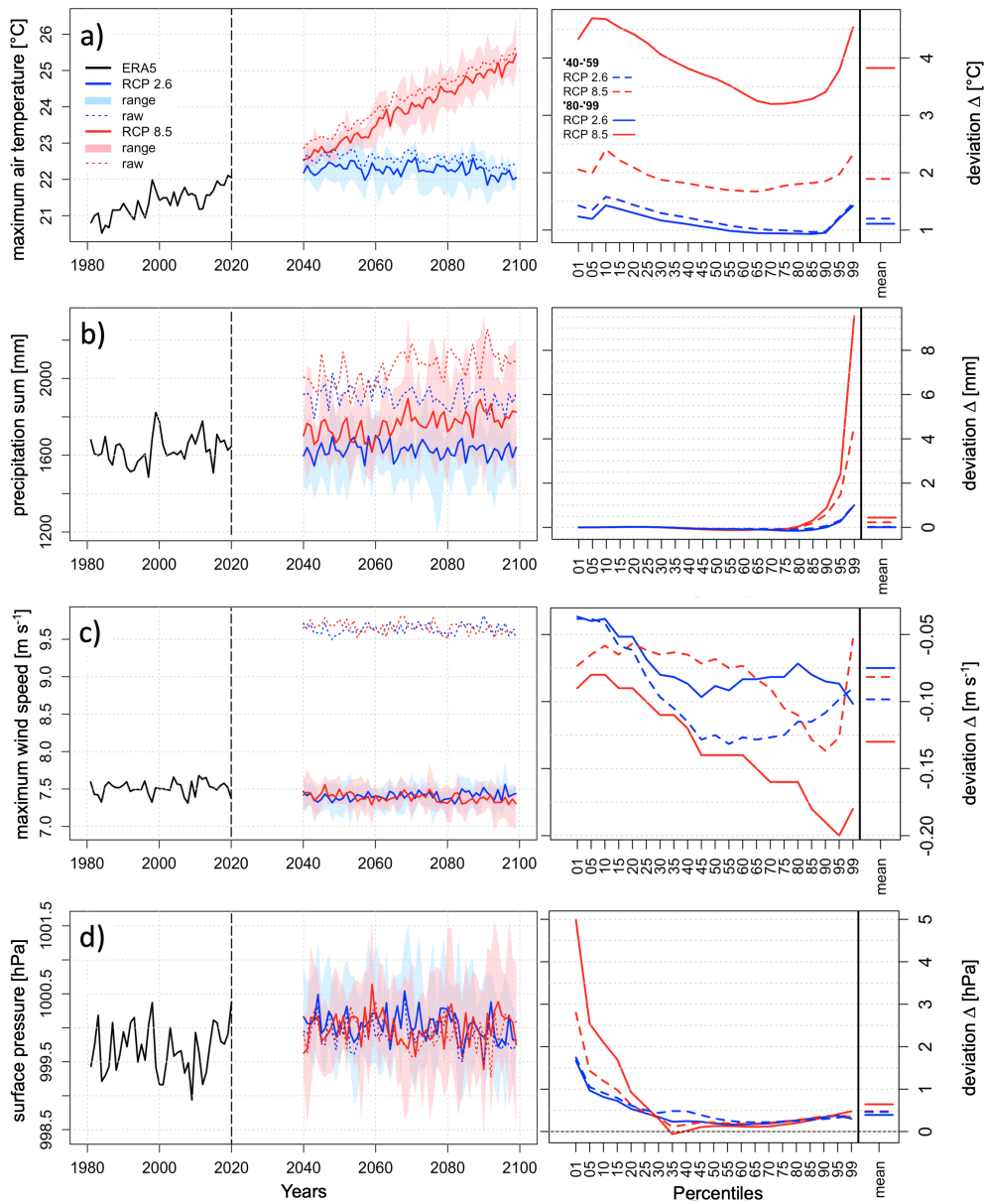
Figure 5. Left: Future projections of annual mean for a) maximum temperature, c) maximum wind speed, d) surface pressure, and annual sum for b) precipitation until 2099. ERA5 reference represented by solid black line, RCP 2.6 in blue, RCP 8.5 in red. Dotted lines are raw output, solid lines are model mean of bias adjusted data, shaded areas indicate range of models. Right: Changes in percentiles for 2040-2059 in dashed lines, 2080-2099 in solid lines. Each with reference to 1981-2000, model minus ERA5.
