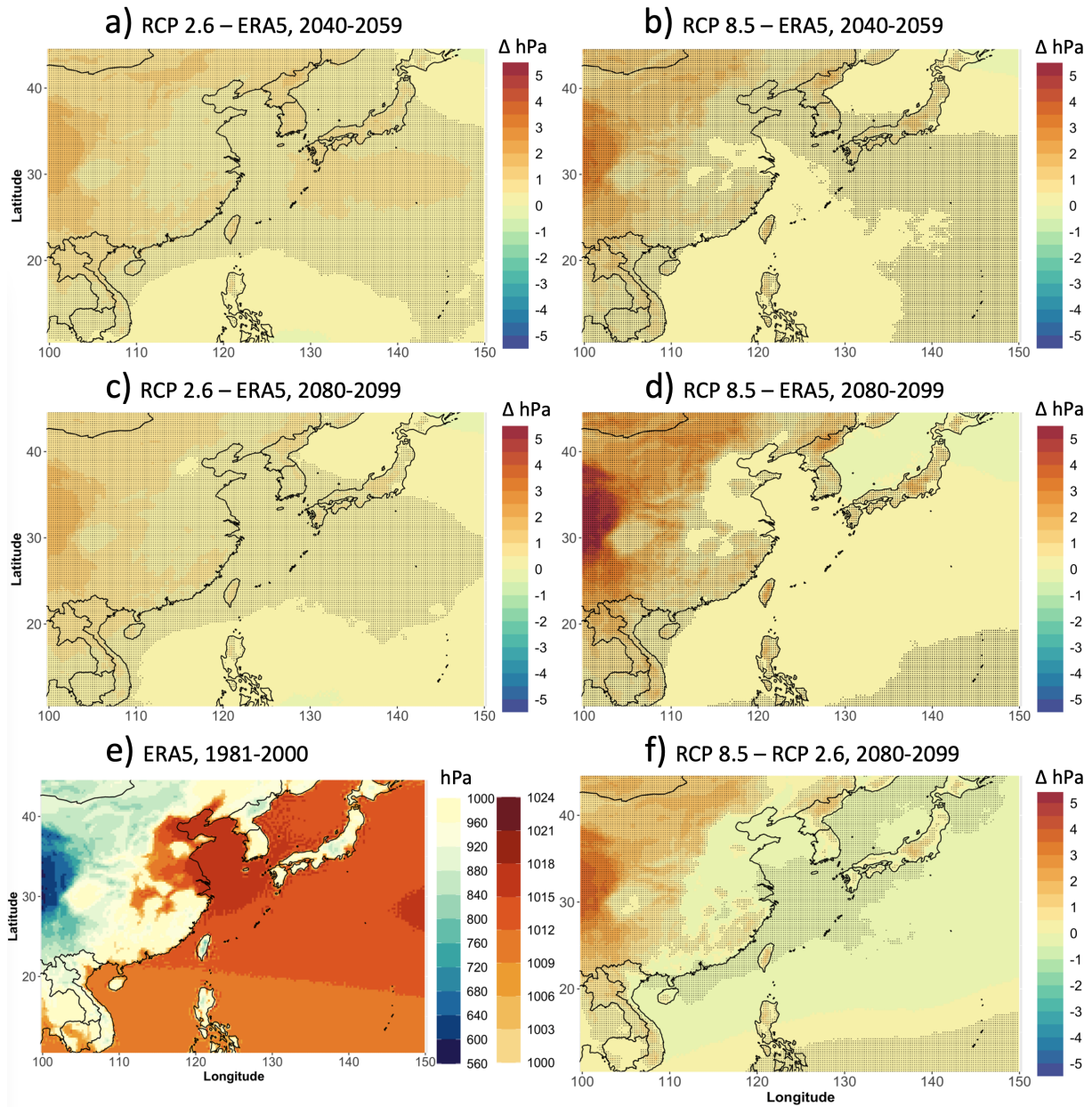
Figure 9. As Figure 6, but for mean daily surface pressure.
