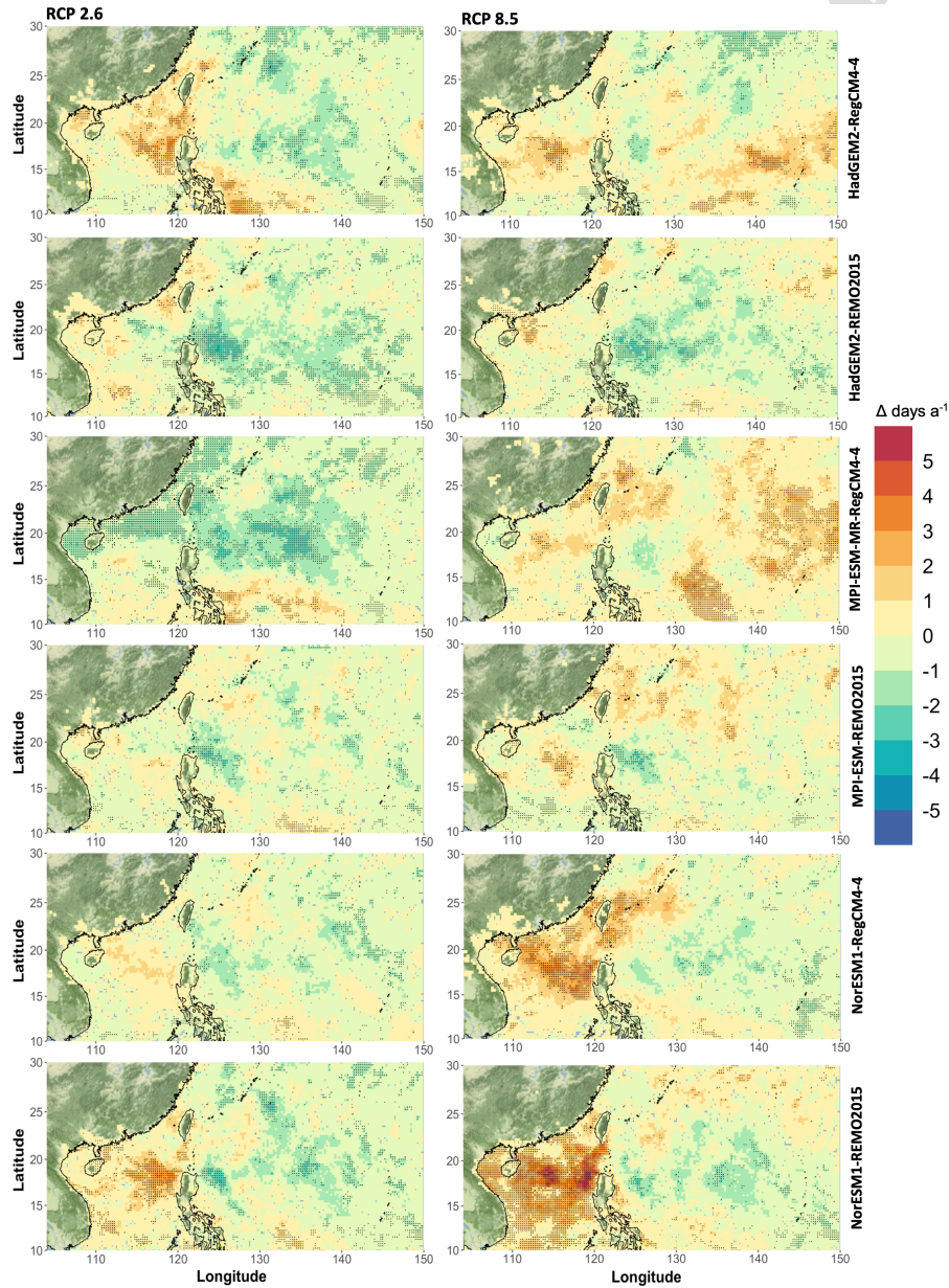
Figure C1. Projected changes in the annual frequency of compound extreme events including tropical cyclone-force winds ( > 17.5 \text{ m s}^{-1} ) and daily precipitation above the 99 th percentile for the included single models. Left side: projected changes in 2080-2099 under RCP 2.6, right side: projected changes in 2080-2099 under RCP 8.5. Rows are single models in accordance with Table 1. Dots indicate statistical significance at \alpha = 0.05 . Please note the varying color scale when comparing to Figure 11.
