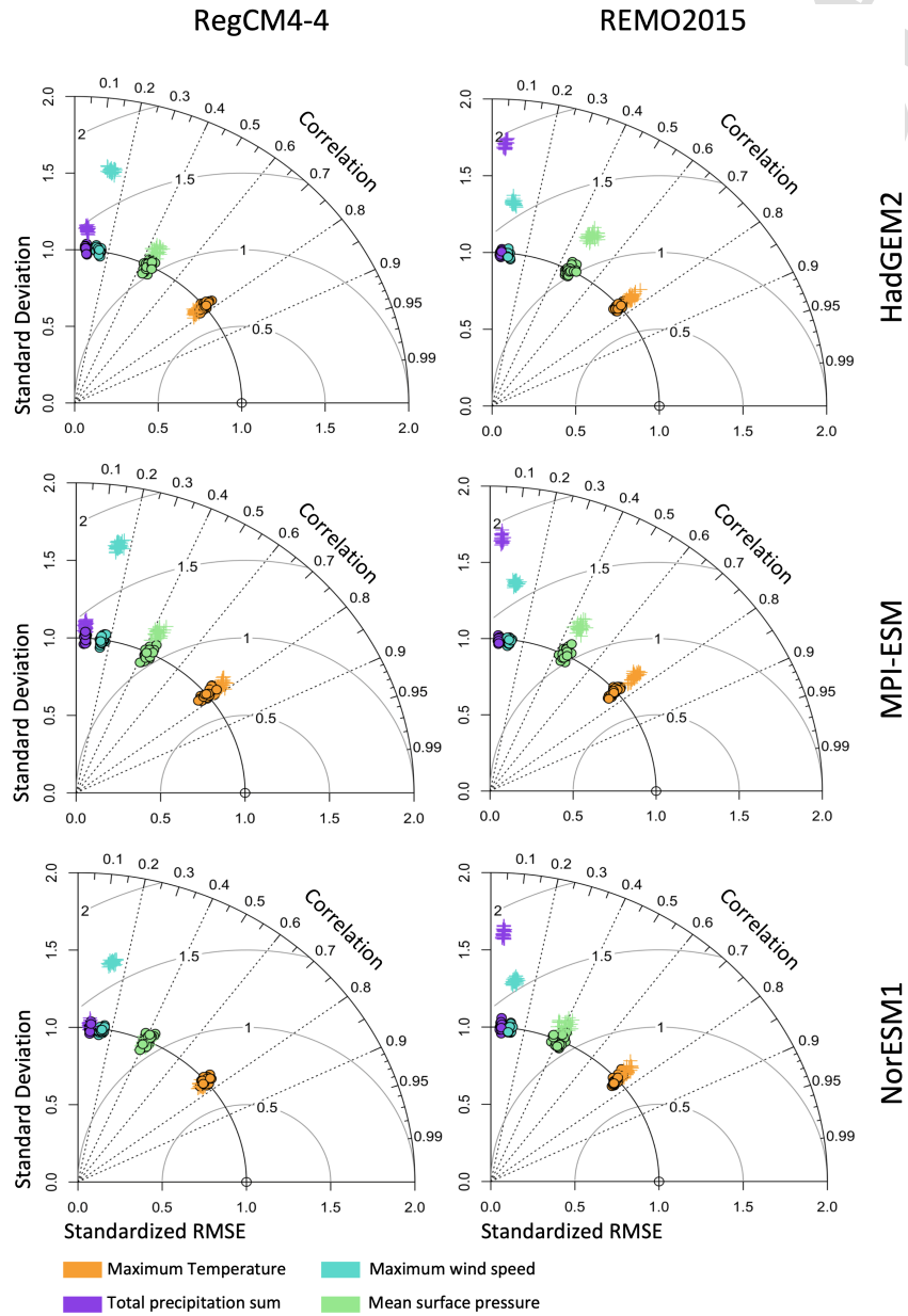
Figure A1. Taylor diagrams to evaluate 30 cross validated ensemble members used for quantile delta mapping (QDM). Each object represents one ensemble member, black outlines depict members of the adjusted data set, colors refer to the inspected variables.
