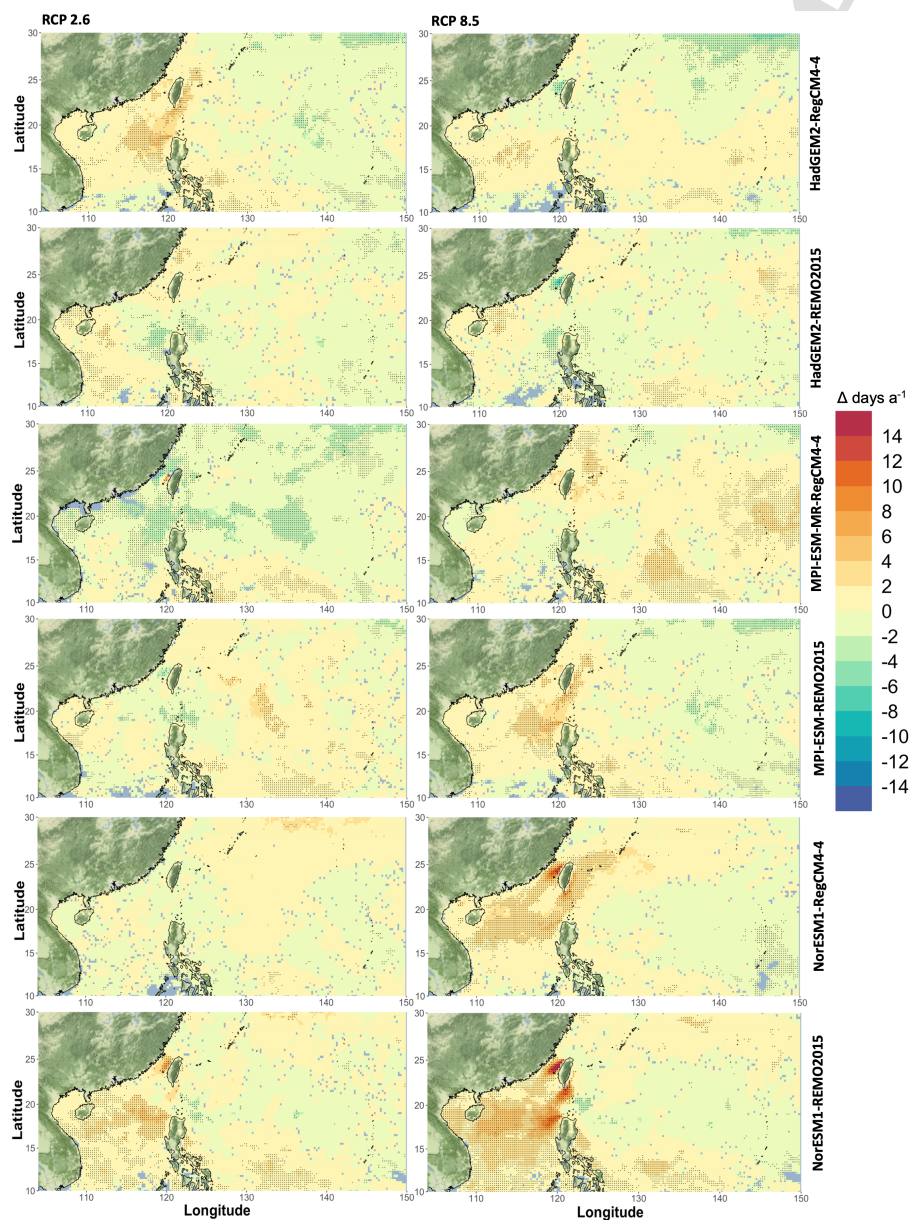
Figure B1. Projected changes in the annual frequency of days with tropical cyclone-force winds > 17.5 \text{ m s}^{-1} for the included single models. Left side: projected changes in 2080-2099 under RCP 2.6, right side: projected changes in 2080-2099 under RCP 8.5. Rows are single models in accordance with Table 1. Dots indicate statistical significance at \alpha = 0.05 . Please note the varying color scale when comparing to Figure 10.
