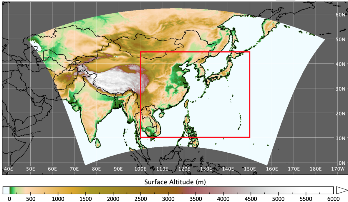
Figure 1. Domain in present study. EAS-CORDEX outer domain in colors, analyzed area enclosed in red.
