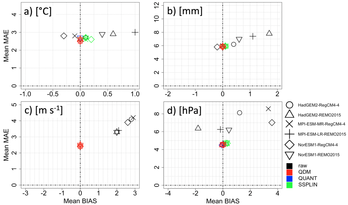
Figure 3. Evaluation of BIAS and MAE within the validation period 1981-2005 for three non-parametric bias adjustment methods (black: raw, green: SSPLIN, blue: QUANT, red: QDM). a) daily maximum air temperature, b) daily precipitation sum, c) daily maximum wind speed, d) daily mean surface pressure.
