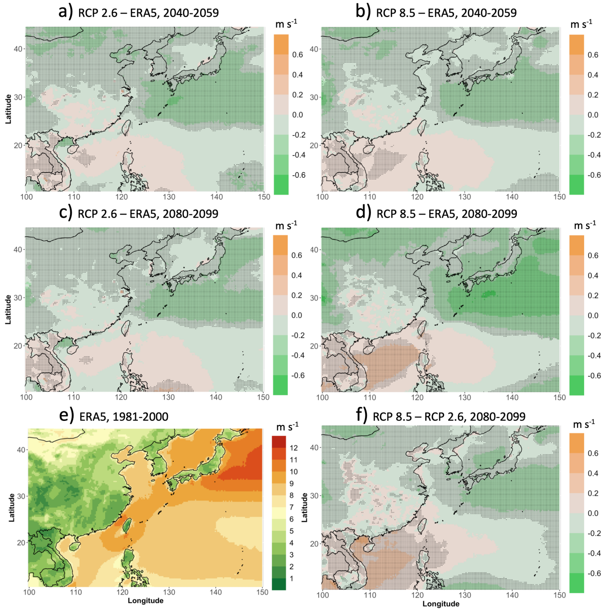
Figure 8. As Figure 6, but for mean daily maximum wind speed.
