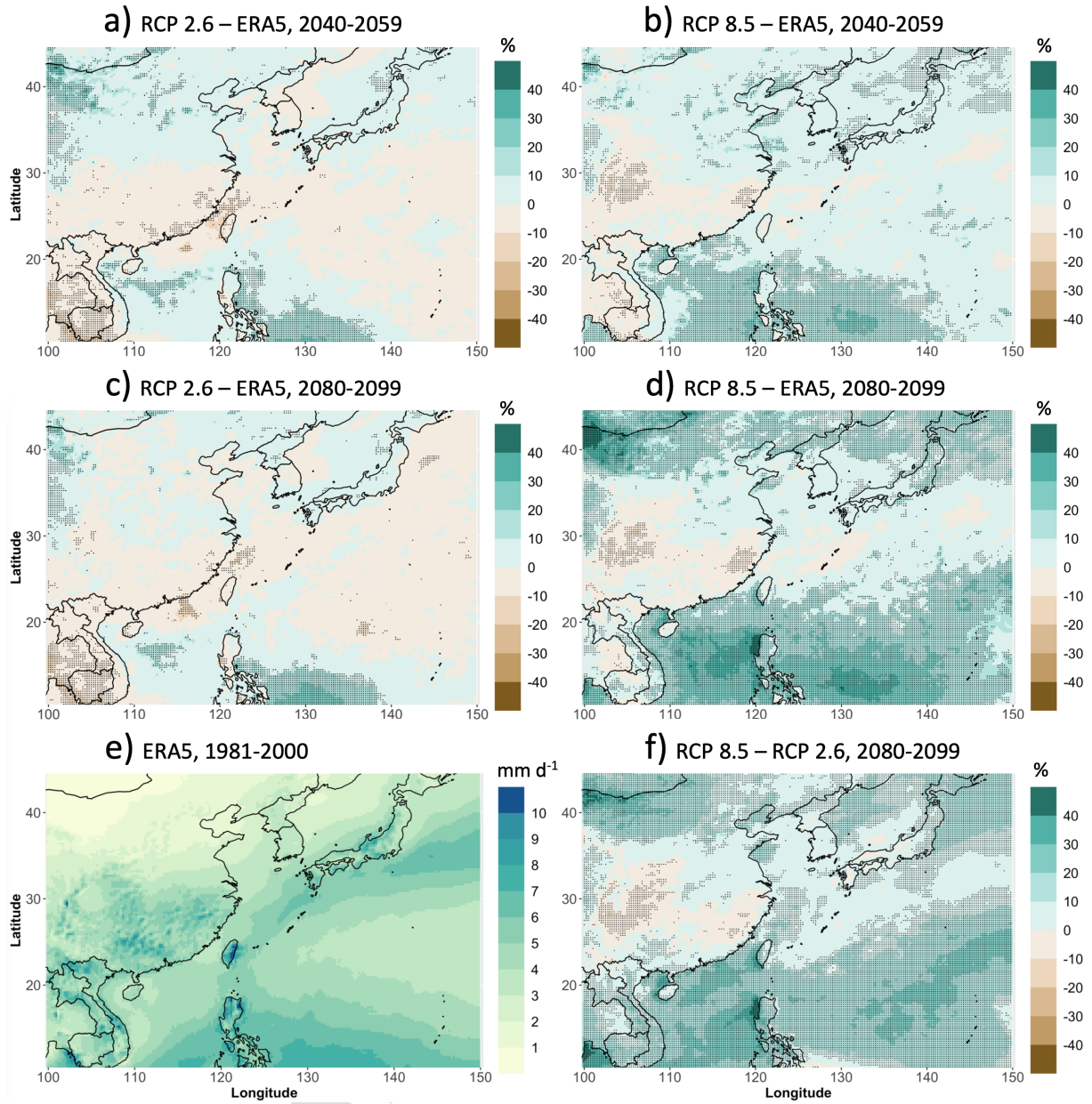
Figure 7. As Figure 6, but for mean daily precipitation.
