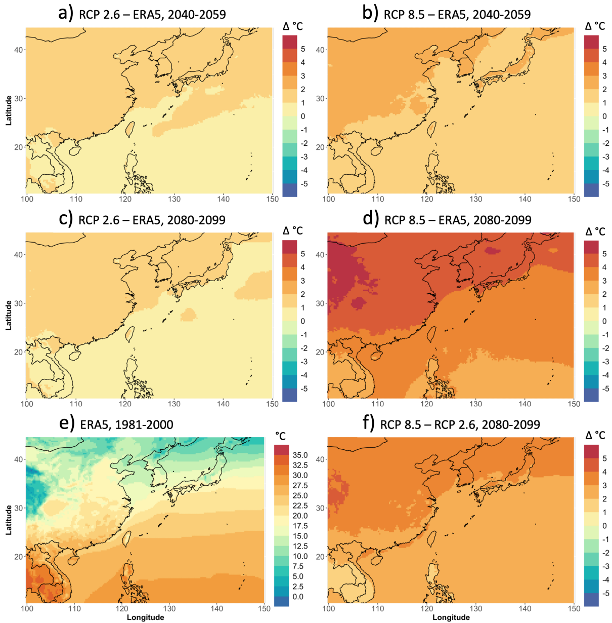
Figure 6. Changes in mean daily maximum temperature in CORDEX model mean. a) RCP 2.6 minus ERA5 (2040-2059), b) RCP 8.5 minus ERA5 (2040-2059), c) RCP 2.6 minus ERA5 (2080-2099), d) RCP 8.5 minus ERA5 (2080-2099), e) ERA5 reference 1981-2000, f) RCP 8.5 minus RCP 2.6. Dots indicate statistical significance at \alpha = 0.05 . Note, that all grid cells for a)-d) and f) show statistical significance for maximum temperature.
