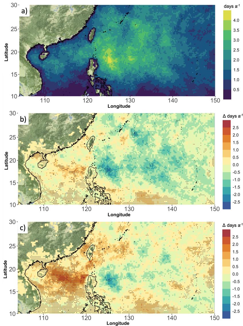
Figure 11. Annual frequency of compound extreme events including tropical cyclone-force winds ( > 17.5 \text{ m s}^{-1} ) and daily precipitation above the 99 th percentile (maximum 1 day lag). a) ERA5 1981-2000, b) projected changes in 2080-2099 for CORDEX model mean under RCP 2.6, c) projected changes in 2080-2099 for CORDEX model mean under RCP 8.5. Dots indicate statistical significance at \alpha = 0.05 .
