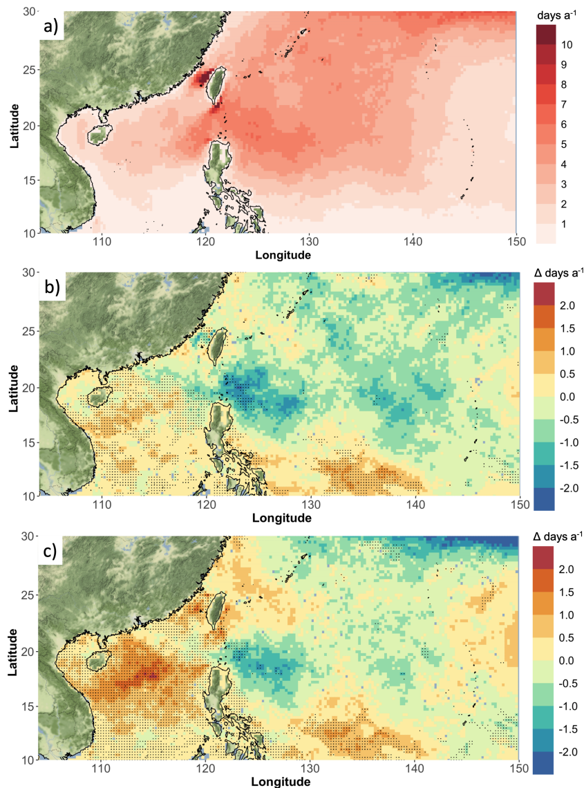
Figure 10. Annual frequency of days with tropical cyclone-force winds > 17.5 \text{ m s}^{-1} . a) ERA5 1981-2000, b) projected changes in 2080-2099 for CORDEX model mean under RCP 2.6, c) projected changes in 2080-2099 for CORDEX model mean under RCP 8.5. Dots indicate statistical significance at \alpha = 0.05 .
