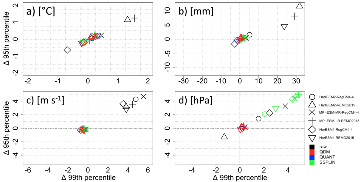
Figure 4. Evaluation of accuracy in the representation of percentiles for three non-parametric bias adjustment methods (black - raw, green - SSPLIN, blue - QUANT, red - QDM). a) daily maximum air temperature, b) daily precipitation sum, c) daily maximum wind speed, d) daily mean surface pressure.
