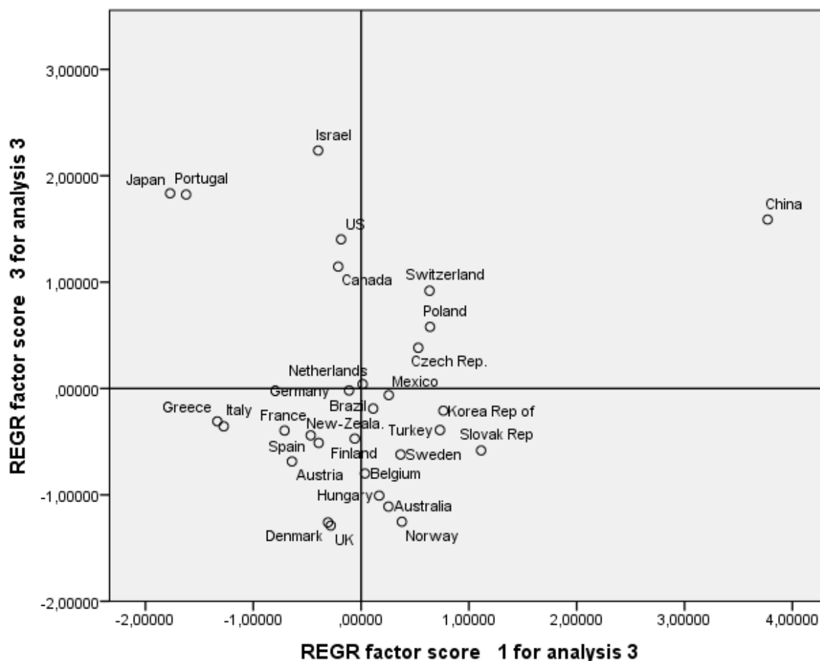
Figure-4-2: Factor Analyses for the REGR factor score 1 and REGR factor score-3 in cases of OECD countries and China
