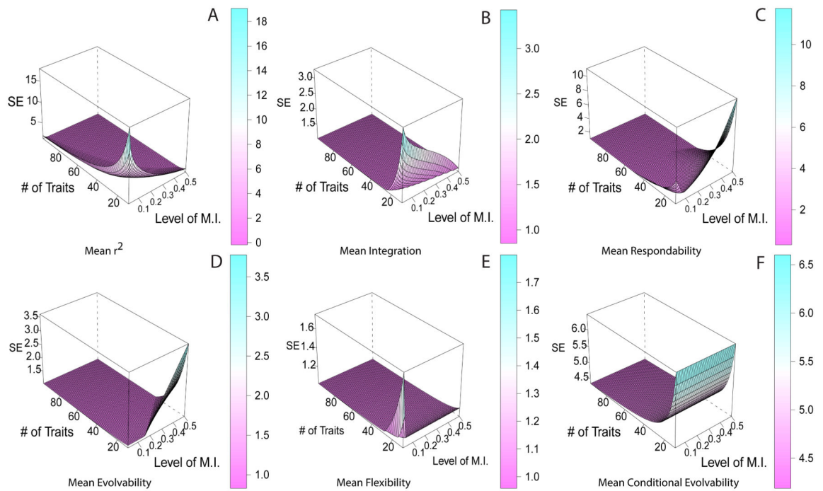
Fig.6. 3D surface plots illustrating the recommended sampling effort necessary to obtain at most 0.05 inaccuracy in the statistics of interest, given different numbers of traits and different population-level magnitudes of integration (level of MI). Sampling effort is measured, in the 3D plots, as the ratio between the number of individuals sampled and the number of traits measured (for illustrative purposes only).
