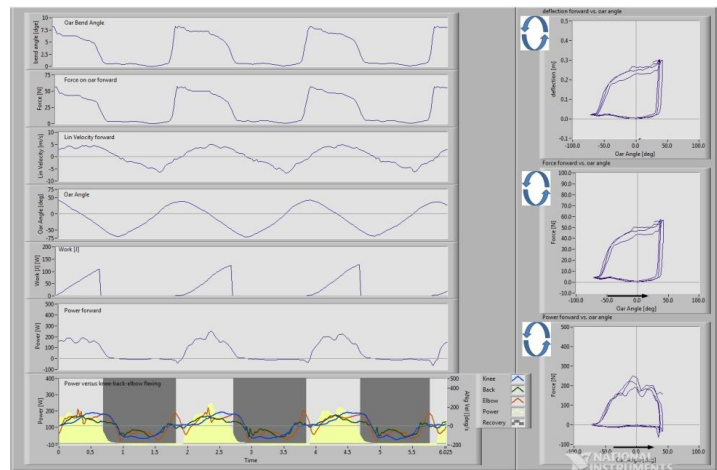
Figure 2: Example of data obtained during actual on water rowing. Left, top down: estimates of oar bend angle, oar forward force, forward velocity, oar angle, work, forward power and power versus knee, trunk and elbow flexion. Right, top down: Deflection forward, forward force, and estimated 'forward' power respectively, all vs. oar angle.
